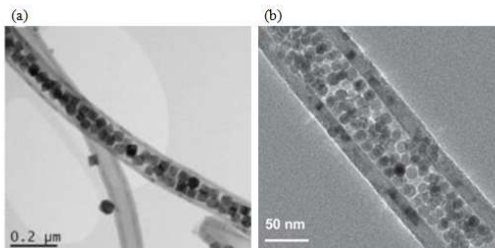
Figure I.20: TEM images of the MWCNT-encapsulated Co-based NPs (141) and Fe 3-x O 4 NPs (142) (reproduced from ref. 141 and 142).
