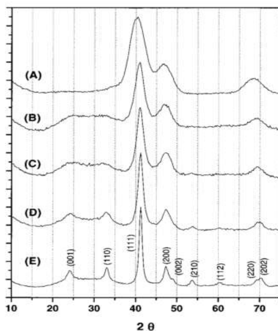
Figure IV.2: Evolution of the FePt phase during annealing. XRD pattern of (a) as-synthesized 4 nm \text{Fe}_{52}\text{Pt}_{48} particle assemblies, and a series of similar assemblies annealed under \text{N}_2 for 30 min at temperature of (b) 450^\circ\text{C} , (c) 500^\circ\text{C} , (d) 550^\circ\text{C} and (e) 600^\circ\text{C} (reproduced from ref 19).
