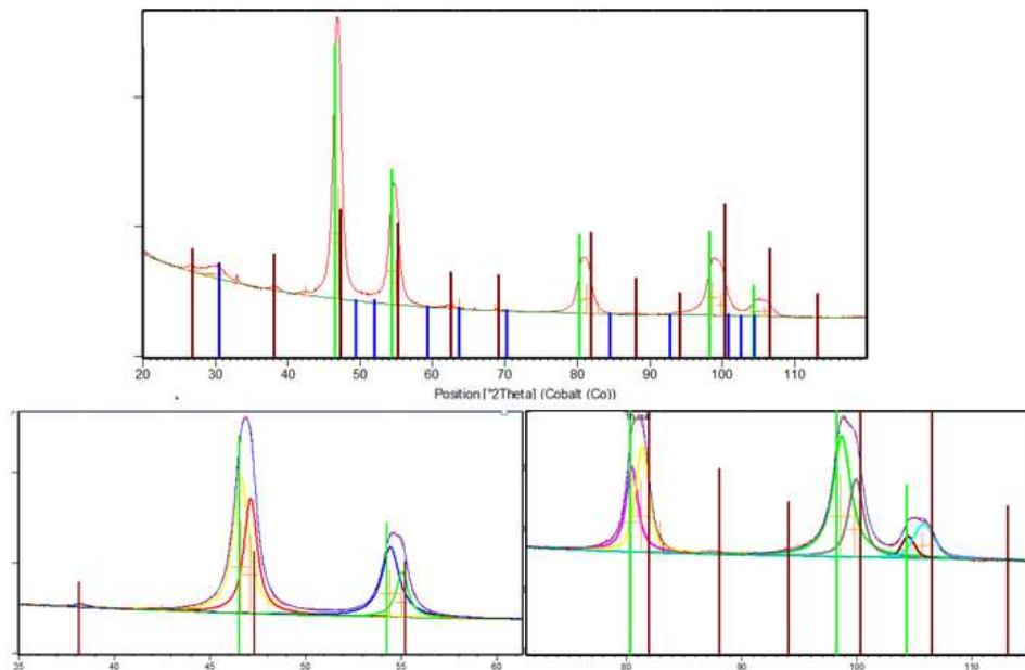
Figure IV.54: XRD pattern of the polyisoprene-coated Fe-Pt NWs at 600°C for one hour. Blue, green and brown lines correspond respectively to carbon, Pt and ordered FePt 3 phases.
