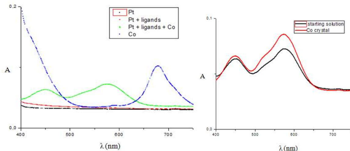
Figure IV.37: UV-visible spectrum. (left) The preparation of the starting solution of "Pt 0.84 Co 2 BBA 2 PPP 2 Tol 100°C 24h "; (right) Comparison between the starting solution and the Co crystal in toluene.
