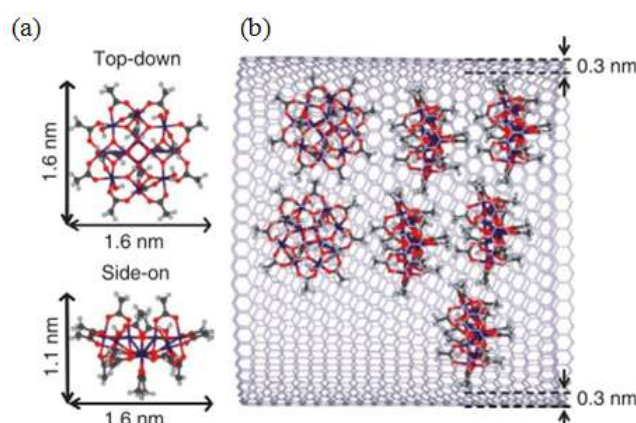
Figure I.11: (a) Size and structure of a SMM \text{Mn}_{12}\text{Ac} molecule; (b) Schematic representation of the innermost layer of a CNT hosting \text{Mn}_{12}\text{Ac} molecules (reproduced from ref.48).
