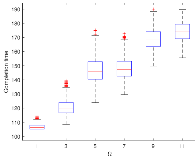
Figure 3.7: Data distribution of 1000 simulations for each \Omega
