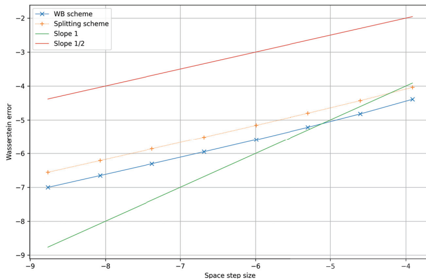
FIGURE 4.3 – Order of convergence of the splitting scheme and the well-balanced scheme for the smooth potential W(x) = \frac{x^2}{2} .
