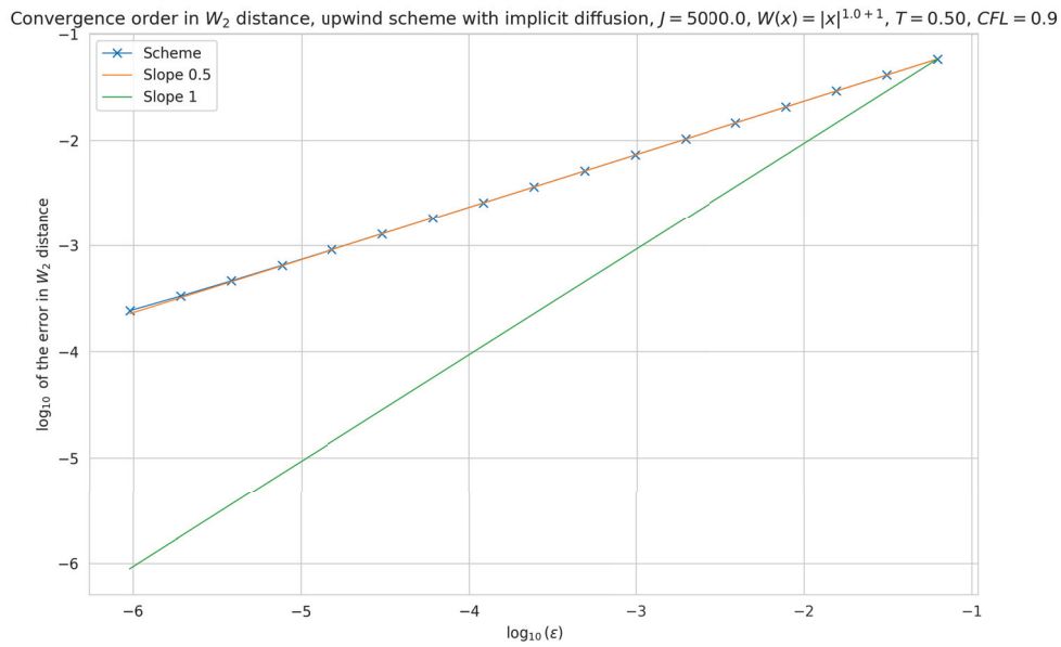
FIGURE 3.1 – Order 1/2 convergence in W_2 distance of \varrho_T^\varepsilon towards \varrho_T for \varrho^{ini}(x) = 2\sqrt{\frac{5}{\pi}}e^{-20x^2} , W(x) = |x|^2 .
