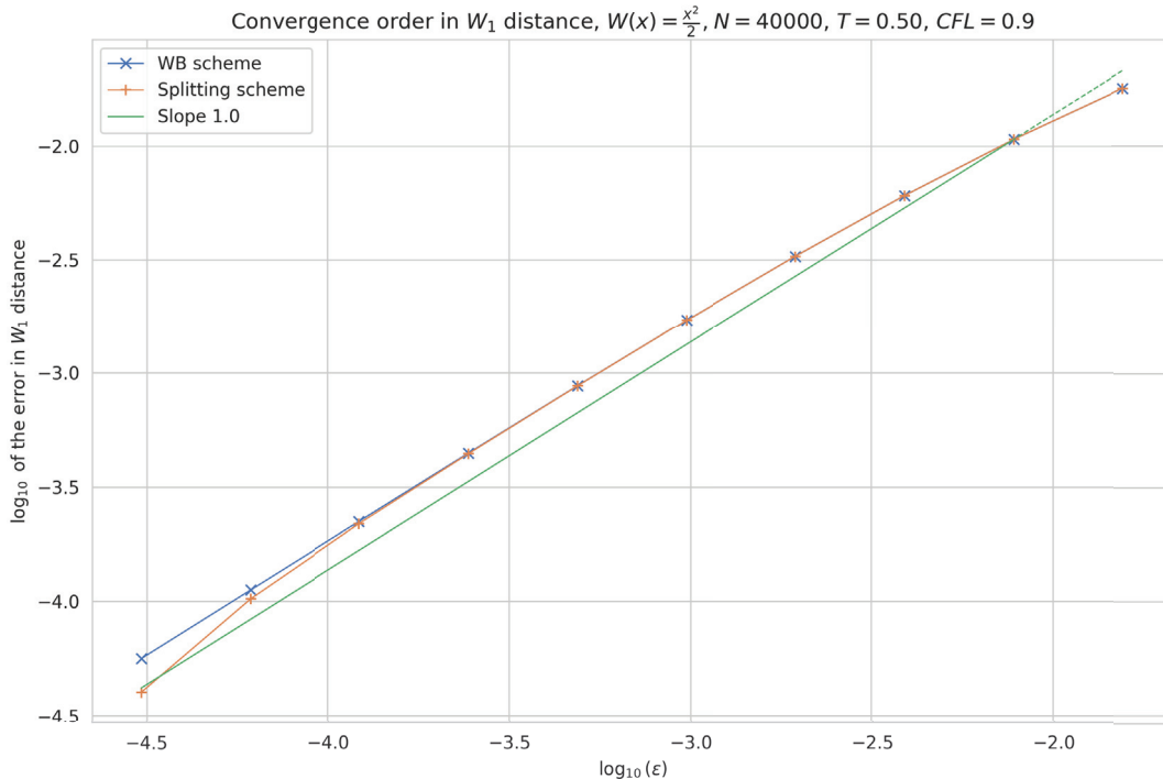
FIGURE 4.7 – Convergence rate w.r.t \varepsilon in W_1 distance, W(x) = \frac{|x|^2}{2} , 40000 cells. Initial datum is one Gaussian bump \varrho_0(x) = 2\sqrt{\frac{5}{\pi}}e^{-20x^2} .
