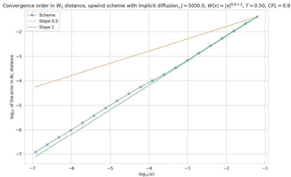
FIGURE 3.2 – Order 1 convergence in W_1 distance of \varrho_T^\varepsilon towards \varrho_T for \varrho^{ini}(x) = 2\sqrt{\frac{5}{\pi}}e^{-20x^2} , W(x) = |x| .
