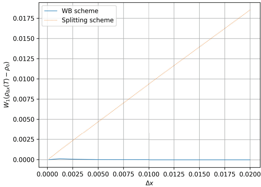
FIGURE 4.5 – Distance to the equilibrium for the splitting scheme and the well-balanced scheme and for the pointy potential W(x) = \frac{|x|}{2} .
