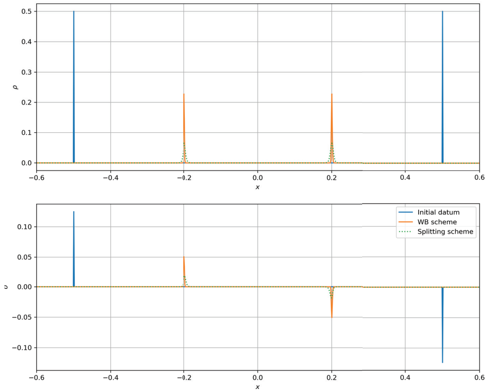
FIGURE 4.2 – Dynamics of two Dirac masses for the potential W(x) = \frac{|x|}{2} in time T = 1.2 .
