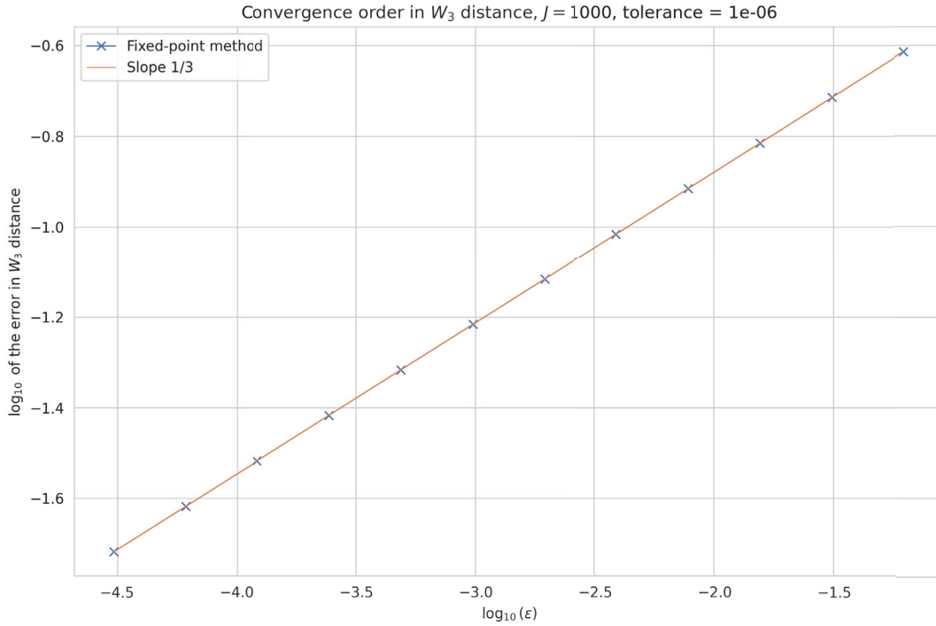
FIGURE 3.5 – O(\varepsilon^{1/3}) convergence in W_3 distance of \varrho^\varepsilon towards \delta_0 , W(x) = |x|^3 . The initial density is the centered Gaussian 2\sqrt{\frac{5}{\pi}}e^{-20x^2} .
