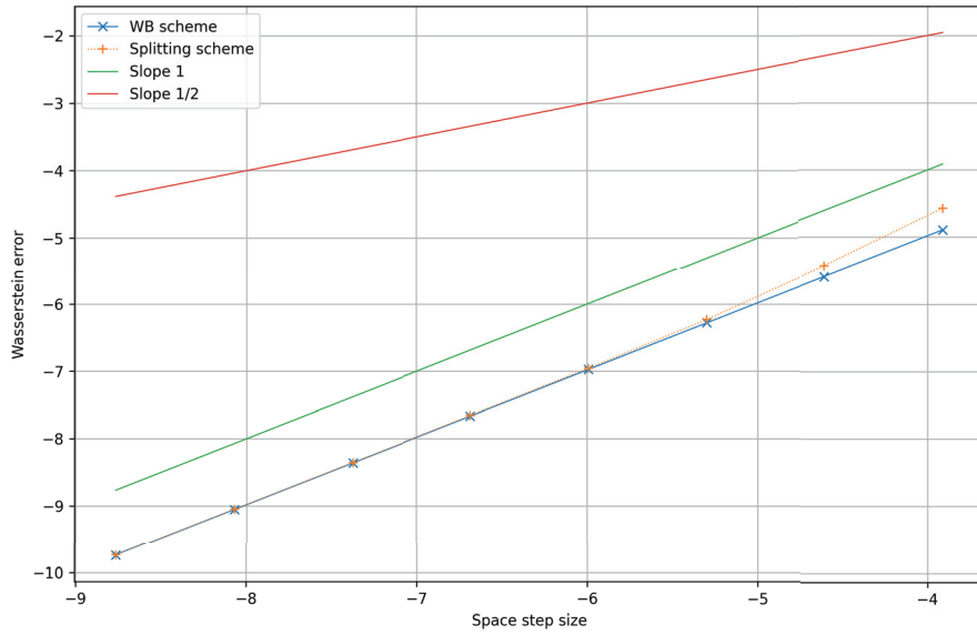
FIGURE 4.4 – Order of convergence of the splitting scheme and the well-balanced scheme for the pointy potential W(x) = \frac{|x|}{2} .
