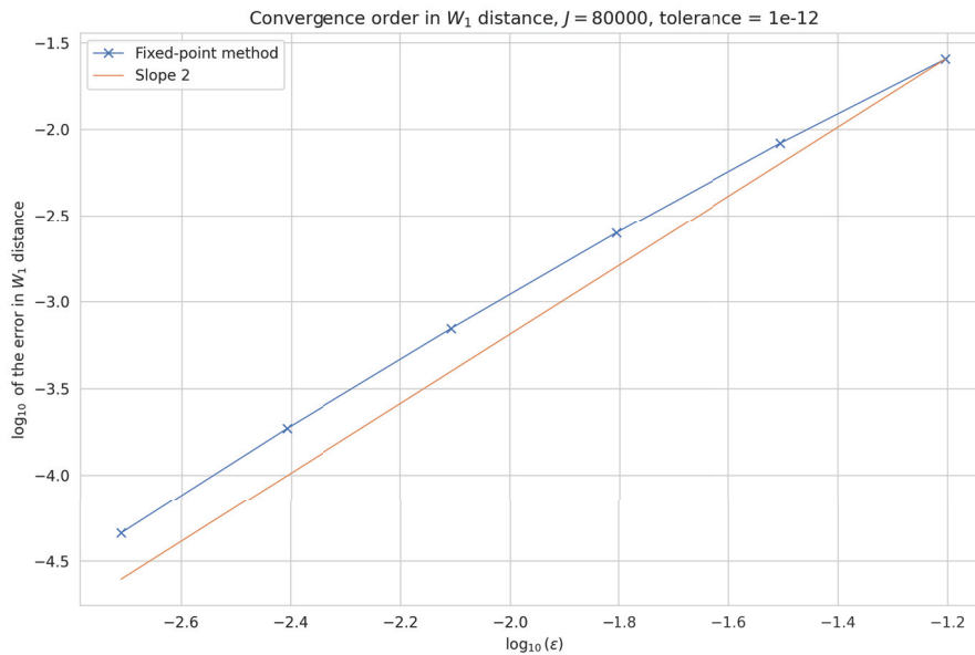
FIGURE 3.4 – Order of convergence in W_1 distance of \varrho^\epsilon towards \delta_0 , for the non-Lipschitz potential W(x) = \sqrt{|x|} + |x| . The initial density is the centered Gaussian 2\sqrt{\frac{5}{\pi}}e^{-20x^2} .
