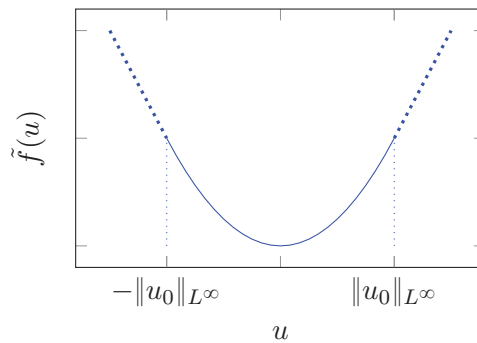
FIGURE 4.1 – The modified flux \tilde{f}
