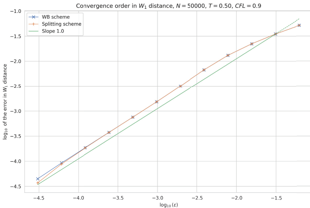
FIGURE 4.6 – Convergence rate w.r.t \epsilon in W_1 distance, W(x) = \frac{|x|}{2} , 50000 cells. Initial datum is one Gaussian bump \varrho_0(x) = 2\sqrt{\frac{5}{\pi}}e^{-20x^2} .
