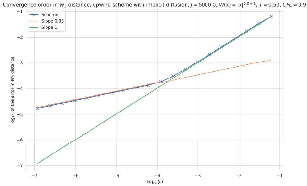
FIGURE 3.3 – Order 1/3 convergence in W_3 distance, for small \epsilon , of \varrho_T^\epsilon towards \varrho_T for \varrho^{ini}(x) = 2\sqrt{\frac{5}{\pi}}e^{-20x^2} , W(x) = |x| .
