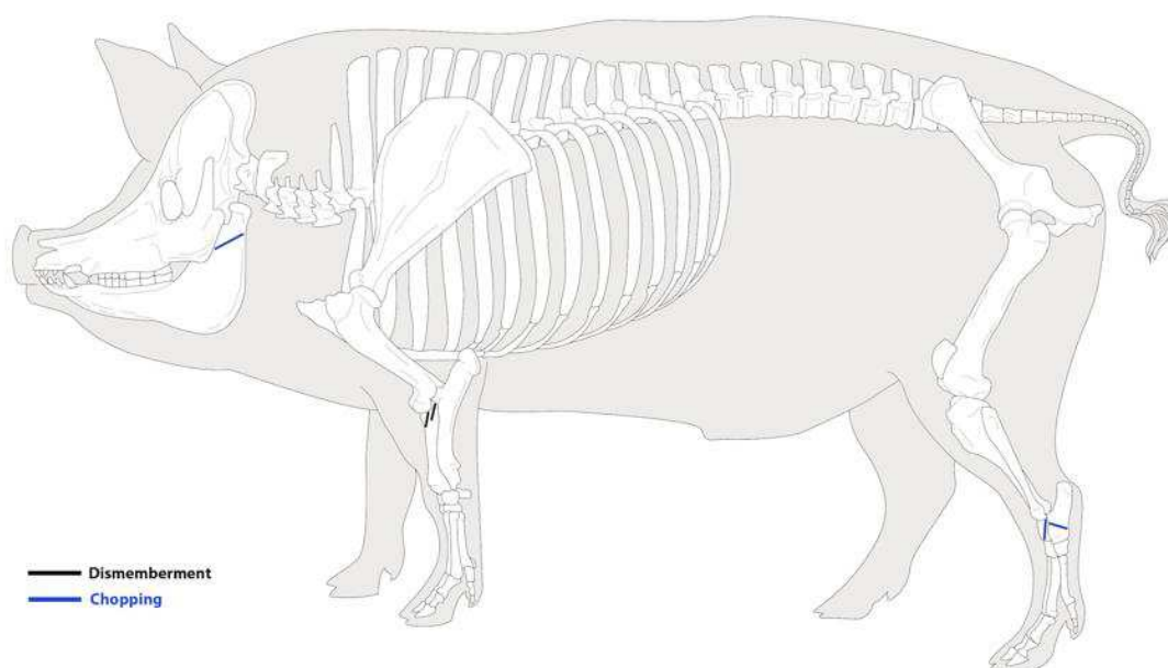
Fig. 3.136. Pig bones displaying butchery marks in EIA Kastri (Appendix III: Table III.11), (©1996 ArcheoZoo.org)
