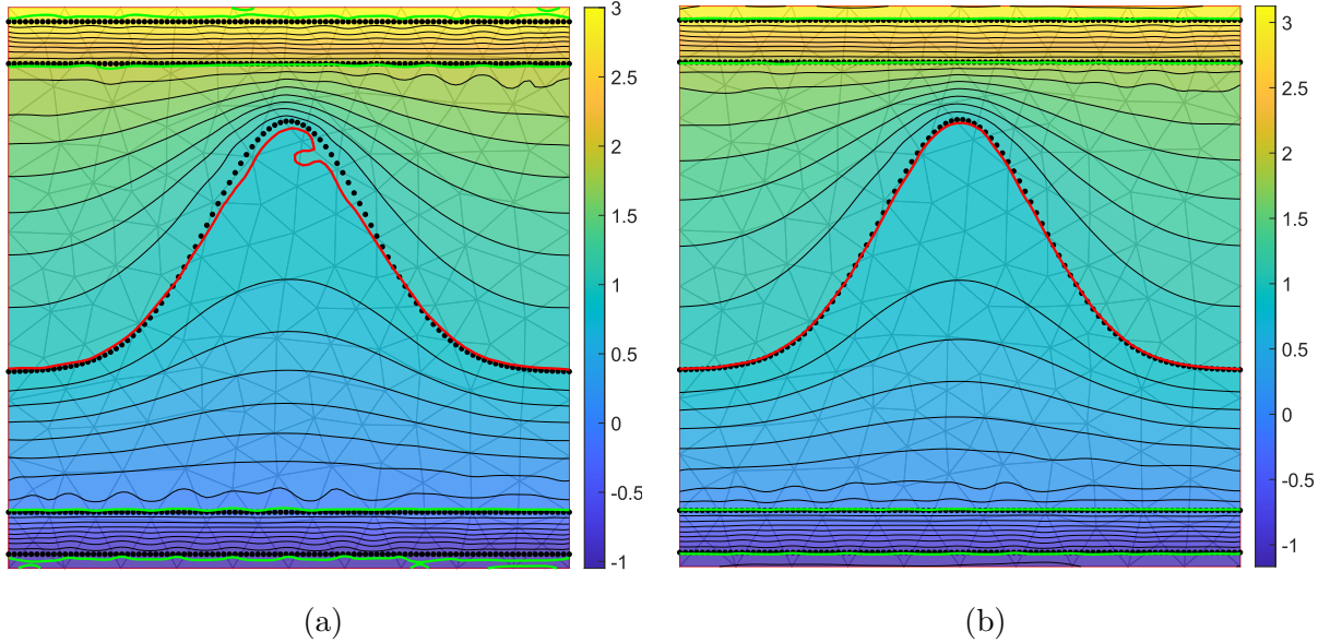
Figure 4.1: Smoother harmonic solution obtained by adding the Hessian energy term, and discretized using the PS-splines. (a) Harmonic solution of Eq. (3.61) ( \lambda = 1 ). (b) Smooth harmonic solution of Eq. (4.3) ( \lambda = 1, \mu = 1 ).
