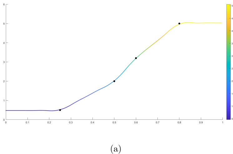
Figure 3.16: 1D interpolation using Dirichlet energy.
