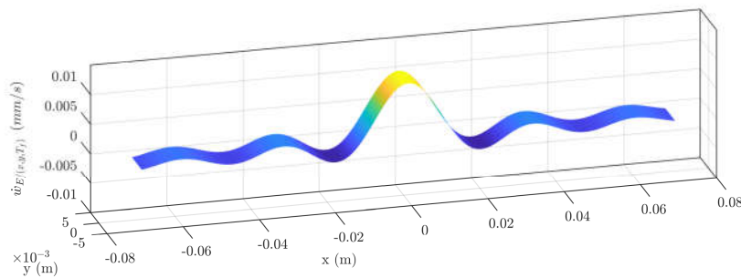
FIGURE 2.2: Example desired spatial vibration velocity form \dot{\mathbf{w}}_R(x, T_F)
