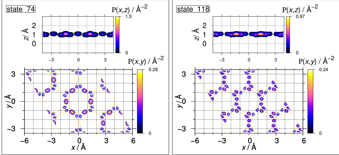
Figure 4.10: Two-dimensional representation of the RPD of eigenstates 74 (left hand side) and 118 (right hand side), lying in sub-levels 7.a and 10.a, respectively. See also the caption of figure 4.4.
