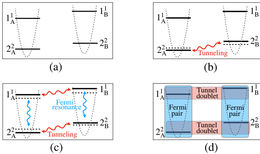
Figure C.3: Schematic representation showing the tunnel doublets and Fermi pairs that can be formed between a quadruplet of states.
