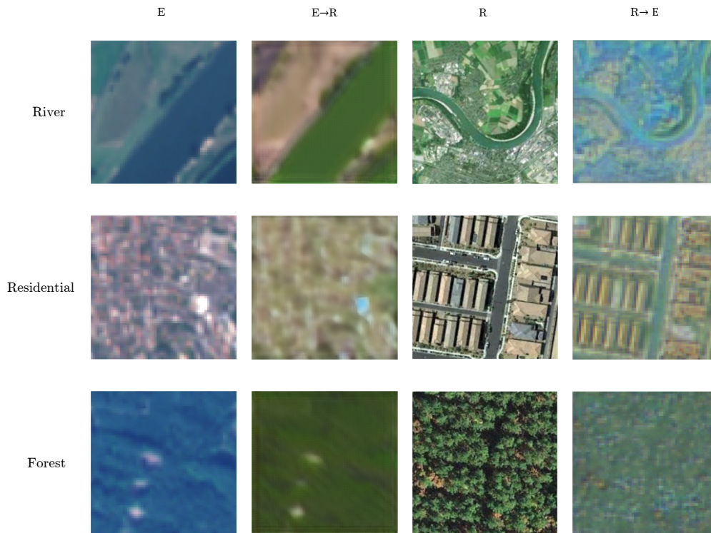
Figure 4.11: The translation of images with the unsupervised CycleGAN for HDA. First column — original Eurosat images (E). Second column — Eurosat images translated to RESISC45 (E→R). Third column — original RESISC45 images (R). Fourth column — RESISC45 images translated to EuroSAT.
