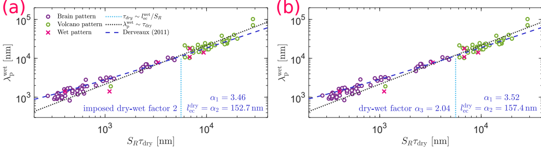
FIG. A.6. Fit of the ratio between swollen and dried wavelength in the thin-film regime. Expected wavelength \lambda_{\text{wet}} when swollen as a function of expected swollen thickness \tau_{\text{wet}} = S_R \tau_{\text{dry}} . The experimental data are fitted with the model of Dervaux and Ber Amar. (a): With two fitting parameters \alpha_1 and \alpha_2 , imposing the ratio between the swollen and dried wavelength in the thin-film regime. (b): With three parameters, \alpha_1 , \alpha_2 and \alpha_3 , the ratio between the swollen and dried wavelength in the thin-film regime being kept as a fitting parameter.
