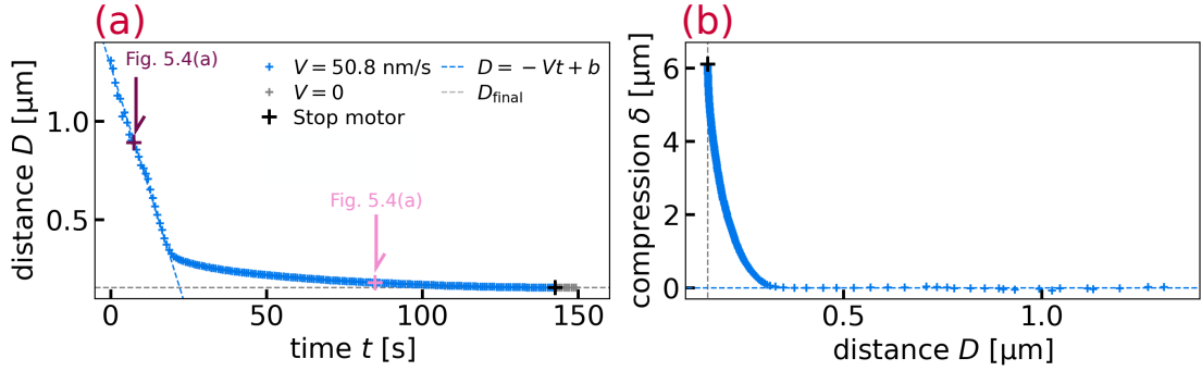
FIG. 5.5. Raw SFA data on a swollen PNIPAM hydrogel. (a): Distance between the two glass surfaces D as a function of time t (blue cross symbols). A linear fit of the initial regime provides a measurement of the approach velocity: V = 50.8 \text{ nm/s} . When no change is visible on the interference pattern, the motor is turned off (black cross symbol). A few more images are recorded (gray cross symbols). (b): Spring compression \delta , as computed in Eq. 5.6 from the data of (a), as a function of the distance between the two glass surfaces D . The black cross symbol is explained in (a).
