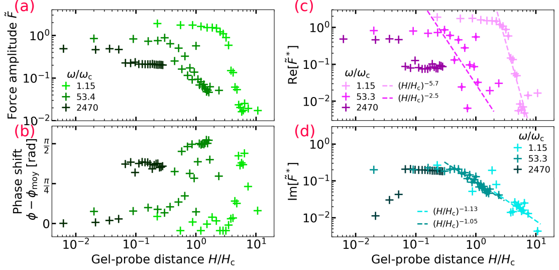
FIG. 4.9. Rescaled force exerted by a hydrogel in oscillatory contactless mode (a): Dimensionless force amplitude \tilde{F} (or modulus of the complex force) as a function of the normalized gel-probe distance H/H_c , for three normalized angular frequencies \omega/\omega_c . (b): Phase shift \phi - \phi_{\text{moy}} (or argument of the complex force) as a function of the normalized gel-probe distance H/H_c , for three normalized angular frequencies \omega/\omega_c . The correction \phi_{\text{moy}} takes into account an intrinsic phase shift of the piezo cube and is described in Sec. 4.2.2.4. (c): Storage component of the dimensionless force (or real part of the complex force) as a function of the normalized gel-probe distance H/H_c , for three normalized angular frequencies \omega/\omega_c . The dashed lines represent power laws fitted on the “+” data points marked by a thick dot, with resulting exponents indicated in the legend. (d): Loss component of the dimensionless force (or imaginary part of the complex force) as a function of the normalized gel-probe distance H/H_c , for three normalized angular frequencies \omega/\omega_c . The dashed lines represent power laws, with resulting exponents indicated in the legend. The color shades used to plot each quantity on each panel are identical to the ones used in Fig. 4.2, to guide the comparison.
