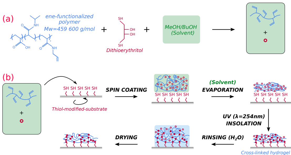
FIG. 2.1. Fabrication of PNIPAM hydrogel films by click-chemistry. (a): A copolymer of P(NIPAM-co-AA) is mixed with DTT (a crosslinker agent), in a mixture of methanol and butanol (solvent). (b): The mixture is deposited onto a functionalized substrate and a uniform layer is obtained by spin-coating. After solvent evaporation, the mixture of melt P(NIPAM-co-AA) and DTT is cured by UV-insolation for 3 hours. The obtained reticulated gel is then rinsed by immersion in water, and dried under ambient air.
