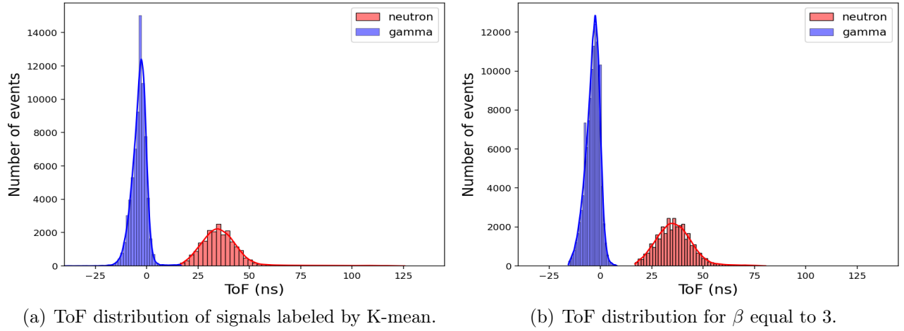
Figure 2.17: Labeling of ToF output vector by K-mean algorithm.
