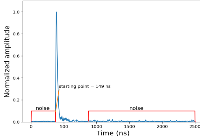
Figure 2.5: Illustration of the noise on a signal obtained using an EJ276 plastic scintillator and a ^{252}\text{Cf} source.
