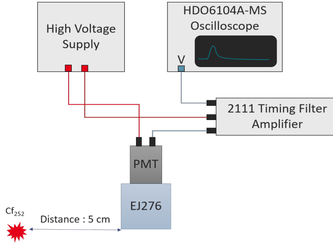
Figure 2.11: The implemented acquisition chain with Op-Amp amplifier.
