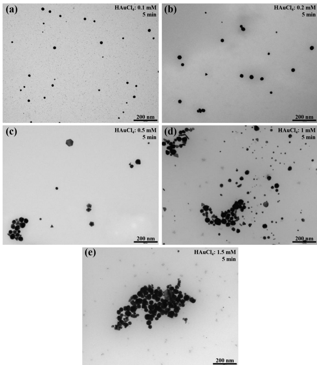
Figure 47. TEM micrographs of the gold nanoparticle solutions after 5 min of plasma exposure with 0.05 mM of PVP at (a) 0.1 mM, (b) 0.2 mM, (c) 0.5 mM, (d) 1 mM, and (e) 1.5 mM of HAuCl 4 concentration.
