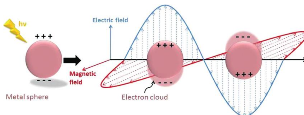
Figure 4. Schematic illustration of the localized surface plasmon resonance (LSPR) of metallic nanoparticles [35].
