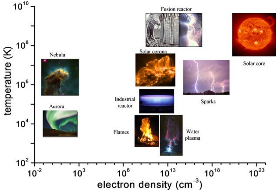
Figure 8. Classification of different plasmas based on their electron density and temperature [89].
