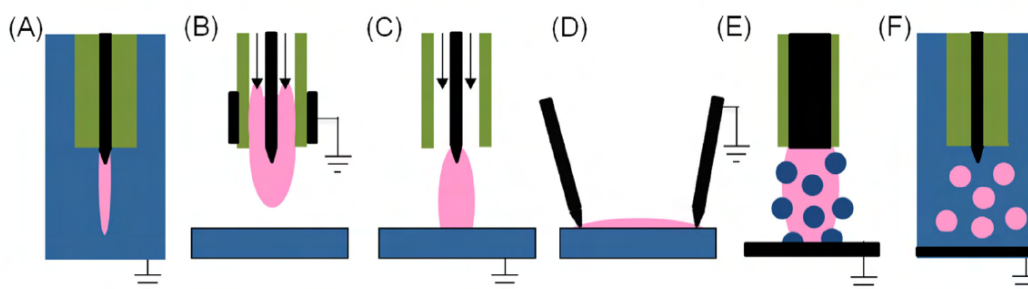
Figure 11. Schematic representation of different discharges: (A) plasma discharge in liquid phase, (B)-(D) plasma discharges above liquid phase, and (E)-(F) multiphase plasma discharges [99].
