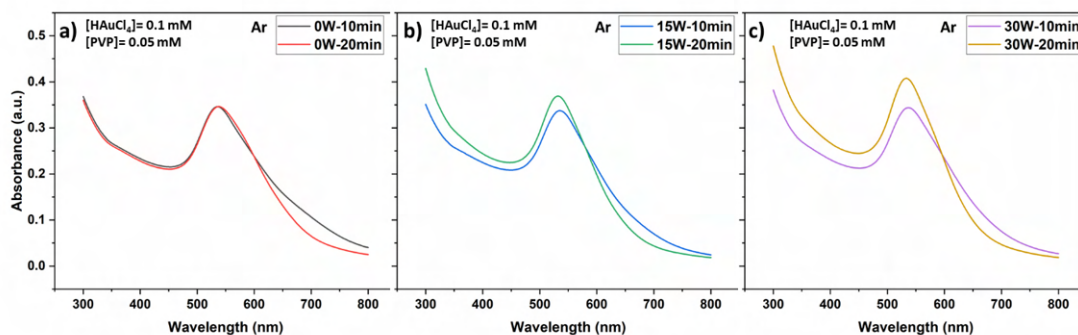
Figure 61. UV-vis absorbance spectra of the obtained gold nanoparticles after 10 and 20 min of argon plasma treatment at a) 0 W, b) 15 W and c) 30 W of RF power.
