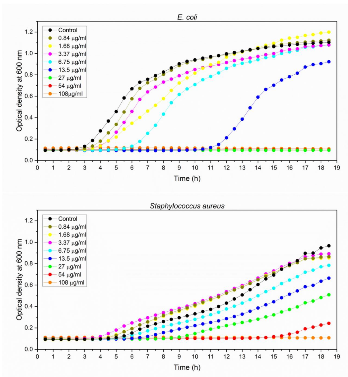
Figure 64. Growth curves of (top) E. coli and (bottom) Staphylococcus aureus cells exposed to different concentrations of silver nanoparticles synthesized by plasma.
