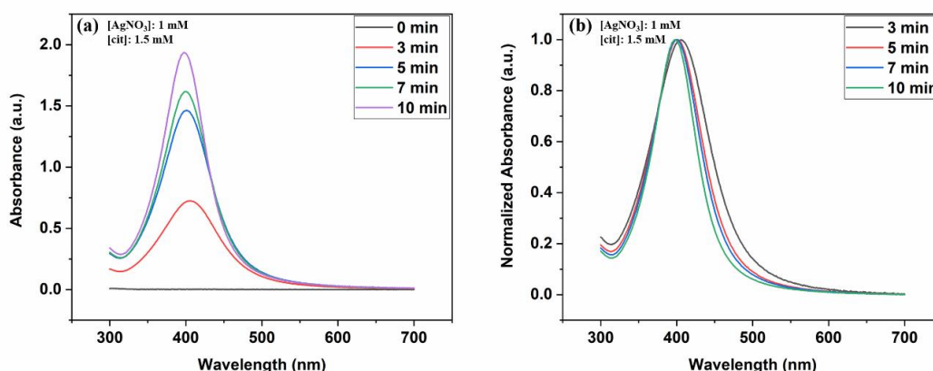
Figure 33. UV-vis (a) absorbance (b) normalized absorbance spectra of the solutions with 1 mM of \text{AgNO}_3 and 1.5 mM of citrate at different plasma exposure durations ranging from 0 (considering 0 as no plasma treatment) to 10 min.
