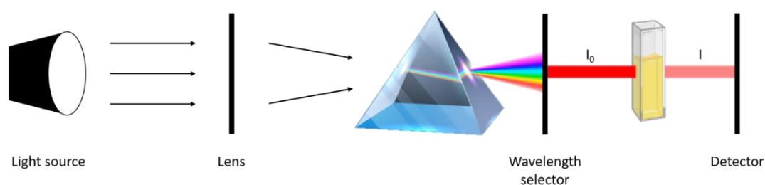
Figure 21. Schematic representation of the instrumentation of a UV-vis spectrophotometer.
