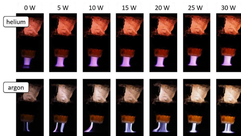
Figure 52. Images of the dual frequency atmospheric pressure plasma jet at different RF power levels with (upper) helium, and (bottom) argon as process gases.
