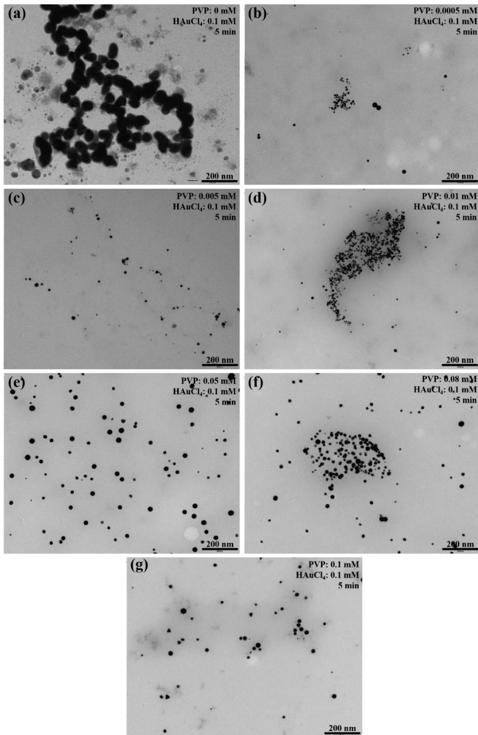
Figure 50. TEM micrographs of the solutions after 5 min of plasma exposure with 0.1 mM of HAuCl 4 at (a) 0 mM, (b) 0.0005 mM, (c) 0.005 mM, (d) 0.01 mM, (e) 0.05 mM, (f) 0.08 mM, and (g) 0.1 mM of PVP concentration.
