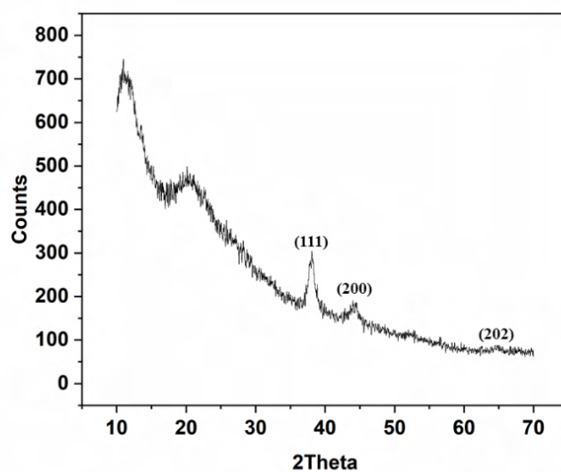
Figure 42. X-ray diffraction pattern of the synthesized AuNPs after 5 min of plasma exposure with 1 mM of \text{HAuCl}_4 and 0.05 mM of PVP.
