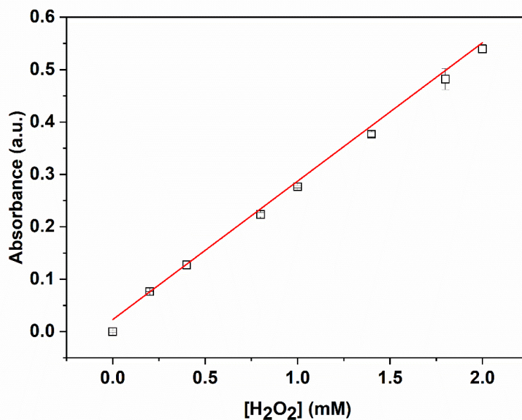
Figure 20. Calibration curve of hydrogen peroxide in liquid phase.
