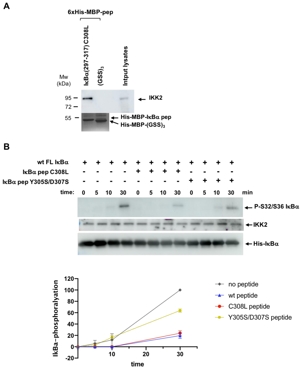
Figure 5. Inhibition assay of endogenous IKK2 activity by \text{I}\kappa\text{B}\alpha synthetic peptides A) Pull-down analysis of the interaction between the \text{I}\kappa\text{B}\alpha(297-317) C308L peptide and endogenous IKK2. The \text{I}\kappa\text{B}\alpha(297-317) C308L peptide was fused to a double 6xHis-MBP tag was expressed in E. coli and purified by \text{Ni}^{2+} -NTA followed by gel filtration chromatography (on a Superdex 200 column). The peptide fusion was then coupled to amylose resin and incubated with clarified extracts of unstimulated HEK cells clarified supernatant. Pull-down samples were migrated on two separate 10% SDS-PAGE gels. Endogenous IKK2 was detected by Western blotting using an antibody anti IKK2 whereas \text{I}\kappa\text{B}\alpha by silver staining. A 6xHis-MBP fusion to a GSS rich peptide was used a negative control. B) Kinase activity experiments using endogenous IKK kinase immunoprecipitated from stimulated HEK293T cells, purified 6His- \text{I}\kappa\text{B}\alpha protein and synthetic peptides encompassing the YDD \Phi X \Phi docking site of \text{I}\kappa\text{B}\alpha (residues 297-317). The peptides tested included the wt \text{I}\kappa\text{B}\alpha sequence and the C308L and Y305S/D307S mutations ( \text{I}\kappa\text{B}\alpha pep C308L and \text{I}\kappa\text{B}\alpha pep Y305S/D307S). A 100-fold excess of synthetic peptide with respect of the \text{I}\kappa\text{B}\alpha substrate concentration (1 \mu\text{M} ) was used in each reaction. ( Upper panel ) Representative Western blot images of the kinase activity experiments. Reactions were migrated on a 10% SDS-PAGE gel and phosphorylated and total \text{I}\kappa\text{B}\alpha proteins were detected using anti P-S32/S36- \text{I}\kappa\text{B}\alpha and anti-His antibodies, respectively. IKK2 was detected using an anti-IKK2 antibody. ( Lower panel ) Quantification of the phosphorylation levels of 6xHis- \text{I}\kappa\text{B}\alpha synthetic peptides. The phospho- \text{I}\kappa\text{B}\alpha bands from the Western blotting analysis were quantified using ImageJ. The phospho- \text{I}\kappa\text{B}\alpha values are normalized to the values obtained in the absence of peptide (no peptide) at 30 min incubation (100%). The data are averages of three independent experiments with error bars representing standard deviation values.
