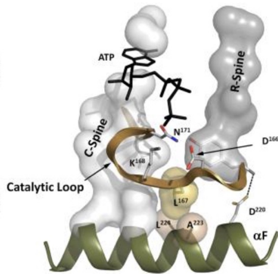
Figure 8. The R- and the C- spines are stably connected to the \alpha F-helix which comes across the kinase core domain. Also, the catalytic region is stabilized by multiple contacts with the \alpha F-helix (taken from Taylor and Kornev, 2011 4 ).
