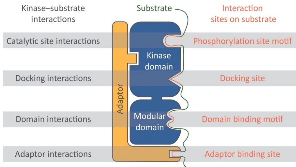
Figure 10. Kinase selectivity relies on different mechanisms that mediate protein-protein interactions. These mechanisms comprise interactions with proximal and distal docking groves in the kinase domain, interactions mediated by modular domains that do not belonging to the core, indirect interactions mediated by scaffold proteins (taken from Miller and Turk, 2018 59 ).
