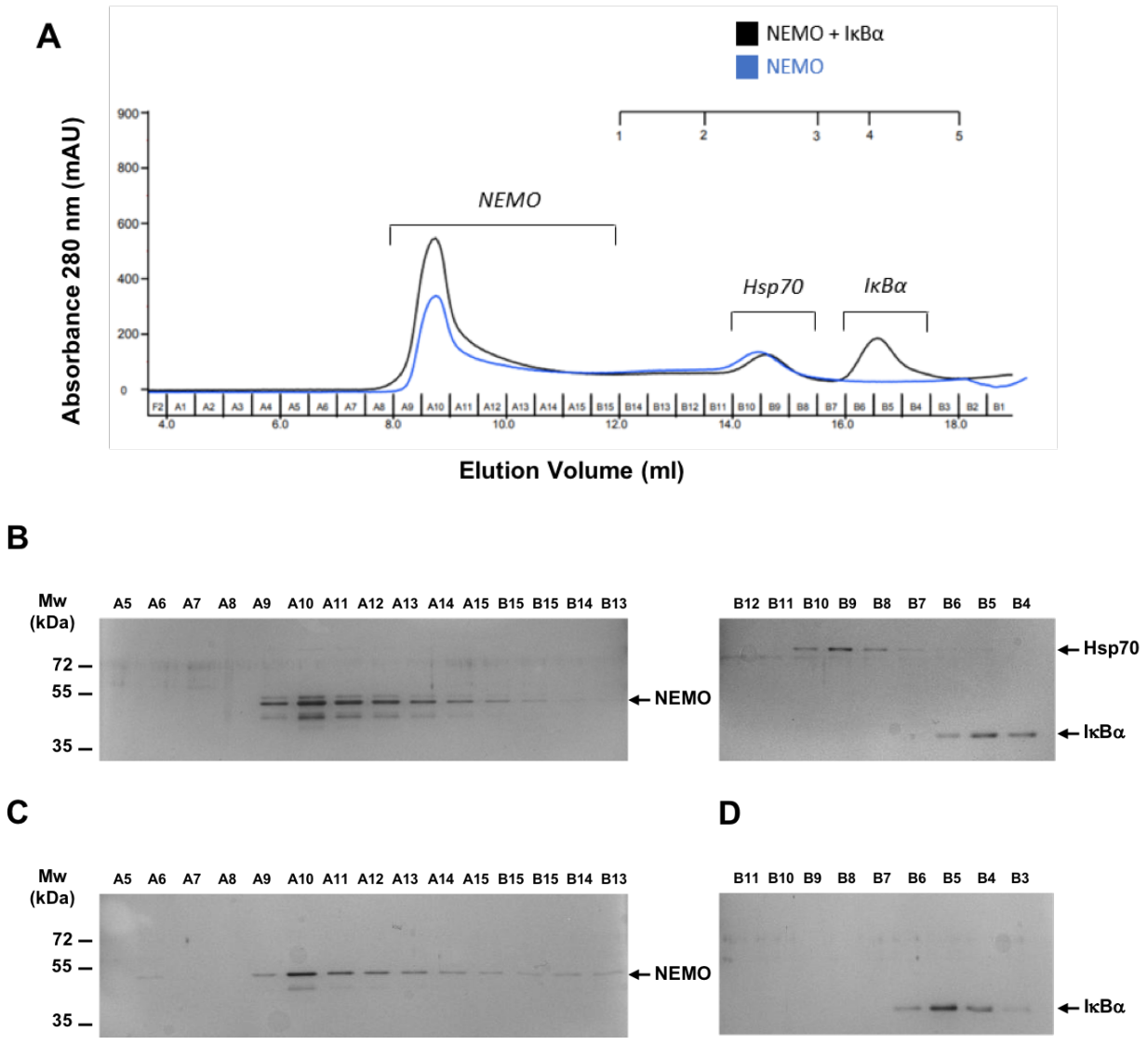
Figure 5. Interaction studies between 6xHis-NEMO and 6xHis-IκBα by gel filtration chromatography. A) Overlay of chromatograms of the NEMO/IκBα 1:1 mixture (black) and of NEMO alone (blue) obtained using a Superose 6 10/300 column. Size markers: 1 - Thyroglobulin (669 kDa); 2 - Ferritin (440 kDa); 3 - Aldolase (158 kDa); 4 - Ovalbumin (44 kDa); 5 - Ribonuclease A (13.7 kDa); 6 - Aprotinin (6.5 kDa). B) 10% SDS-PAGE gel analysis followed by silver nitrate staining of the fractions between 6 and 17.5 ml of the elution volume (A5 to B4) for the NEMO/IκBα mix. C) 10% SDS-PAGE gel analysis followed by silver staining of the 6 to 13 ml elution fractions (A5 to B4) for NEMO alone. D) 10% SDS-PAGE gel analysis followed by silver staining of the 13.5 to 18 ml fractions (B11 to B3) for IκBα alone.
