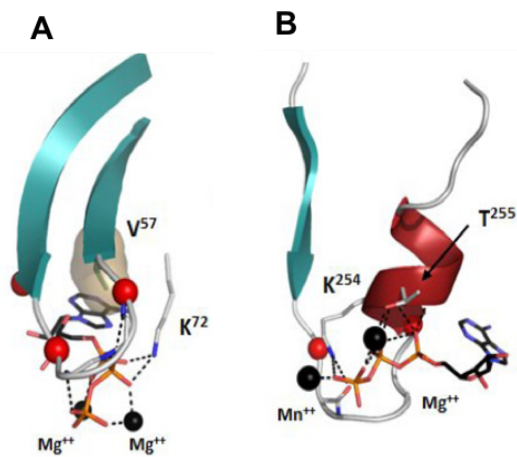
Figure 4. A) The G-loop is included between the \beta -strands 1 and 2 of the N-lobe. It harbors the glycine-rich motif that folds over the ATP, shielding the g-phosphate and orienting the adenine ring. B) The Walker loop (also called P-loop) is found instead of the G-loop (taken from Taylor and Kornev, 2010 57 ).
