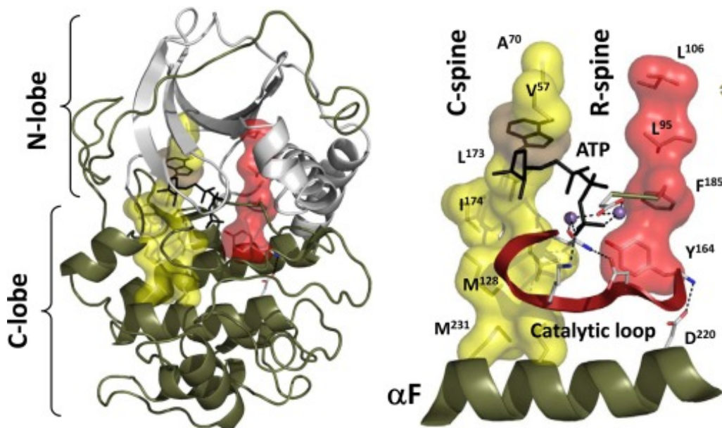
Figure 9. The hallmark of an active kinase domain is the assembly of the R and the C-spines. The R-spine is a transient structure made of 4 hydrophobic residues. R1 and R2 belong to the C-lobe, while R3 and R4 to the N-lobe. R1 comes from the HRD sequence that identifies the beginning of the catalytic loop while R2 from the DFG motif at the beginning of the activation loop. R3 and R4 are found in the \alpha C and \beta 4 strand respectively (taken from Shaw et al., 2014 29 ).
