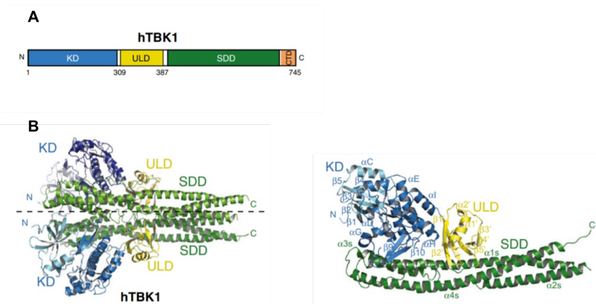
Figure13. A) Domain architecture of TBK1. B) 3D structure of TBK1 showing the dimer and the isolated monomer subunit with the KD domain displayed in blue, the ULD domain in yellow and the SDD domain in green (taken from Larabi et al., 2013 16 ).
