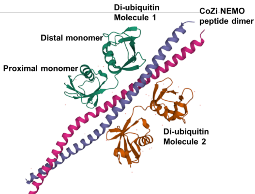
Figure 10. The structure of NEMO CoZi region homodimers bound to two molecules of di-Ub, resolved at 2.7 Å, reveals how linear polyUb chains bind to the UBAN motif. Observing the green di-Ub molecule 1, the monomer atop is the distal, while the lower is the proximal molecule. (PDB: 2ZVO) 14 .
