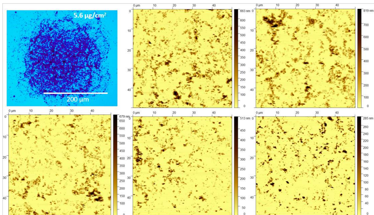
Figure 36 Micrograph and AFM images of 5.6 µg/cm 2 deposit with 15 % Nafion.
