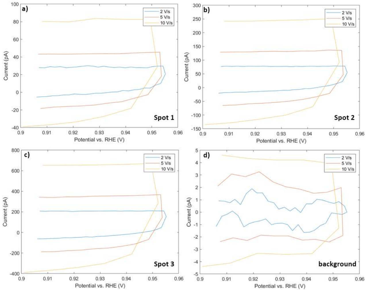
Figure 50 CVs at a potential range of 0.906 V to 0.956 V at scan rates of 2,5 and 10 V/s for a) spot 1, b) spot 2, c) spot 3 and d) the background. Data from the 100x100 \mu\text{m} scan with a 3 \mu\text{m} hopping distance, acquired with a \sim 250 nm pipette.
