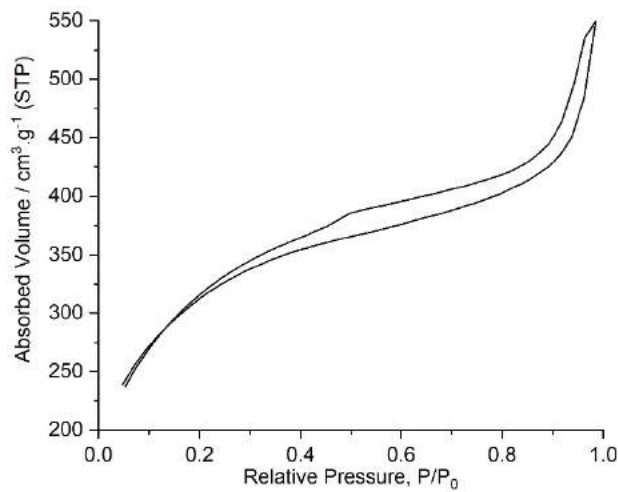
Figure 58 Nitrogen adsorption–desorption BET isotherm. The surface area is 1132 \text{ m}^2\text{g}^{-1} .
