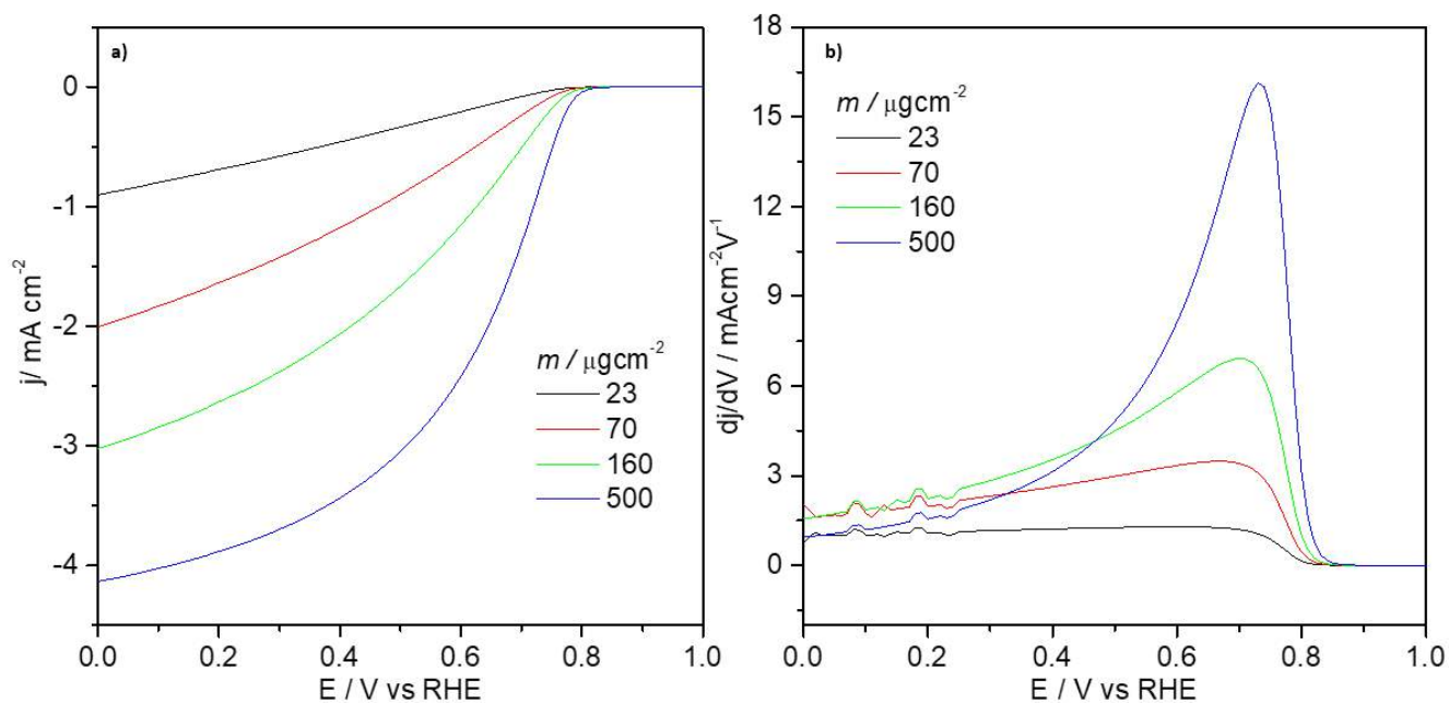
Figure 21 a) Example of simulated voltammograms at different loadings and b) the corresponding simulated derivatives/slopes by Alice Boudet.
