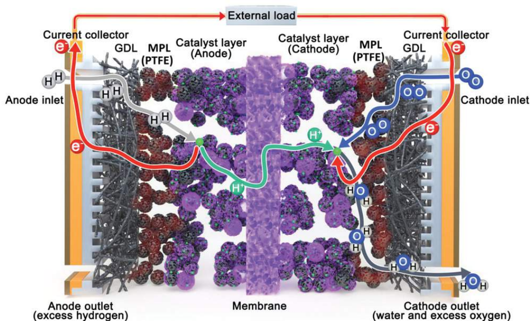
Figure 4 PEMFC scheme. 24
