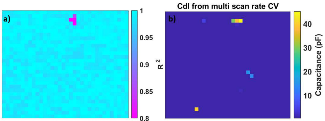
Figure 51 a) Coefficient of determination ( R^2 ) acquired from the fitting of current vs scan rate, b) double layer capacitance C_{dl} acquired from the slope of current vs scan rate. Data from the 100x100 \mu\text{m} scan with 3 \mu\text{m} hopping distance, \sim 250 nm pipette.
