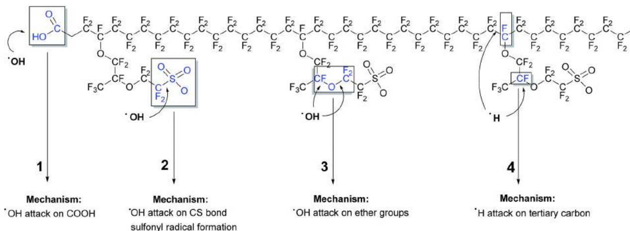
Figure 35 Possible mechanisms of \text{OH}^* radical attack at different functional groups of Nafion structure. 188
