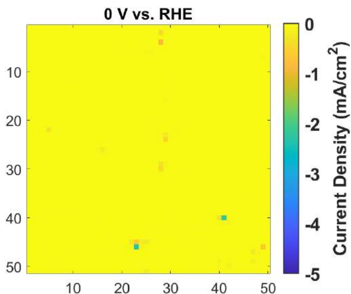
Figure 46 ECSA normalized activity map considering the specific capacitance of BDD ( 3\mu\text{F}/\text{cm}^2 ) rather than the catalyst one. Data from the 40x40 \mu\text{m}^2 scan with a 0.8 \mu\text{m} hopping distance, acquired with a \sim 150 nm pipette.
