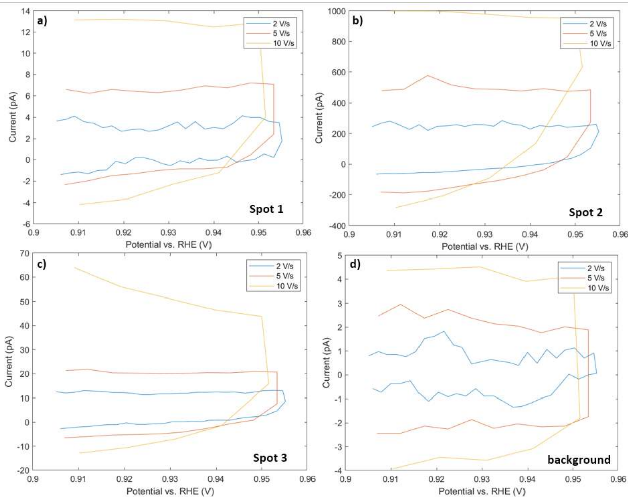
Figure 42 CVs at a potential range of 0.906V to 0.956 V at scan rates of 2,5 and 10 V/s for a) spot 1, b) spot 2, c) spot 3 and d) the background. Data corresponds to the 40x40 \mu\text{m} scan with a 0.8 \mu\text{m} hopping distance, acquired with a \sim 150 nm pipette.
