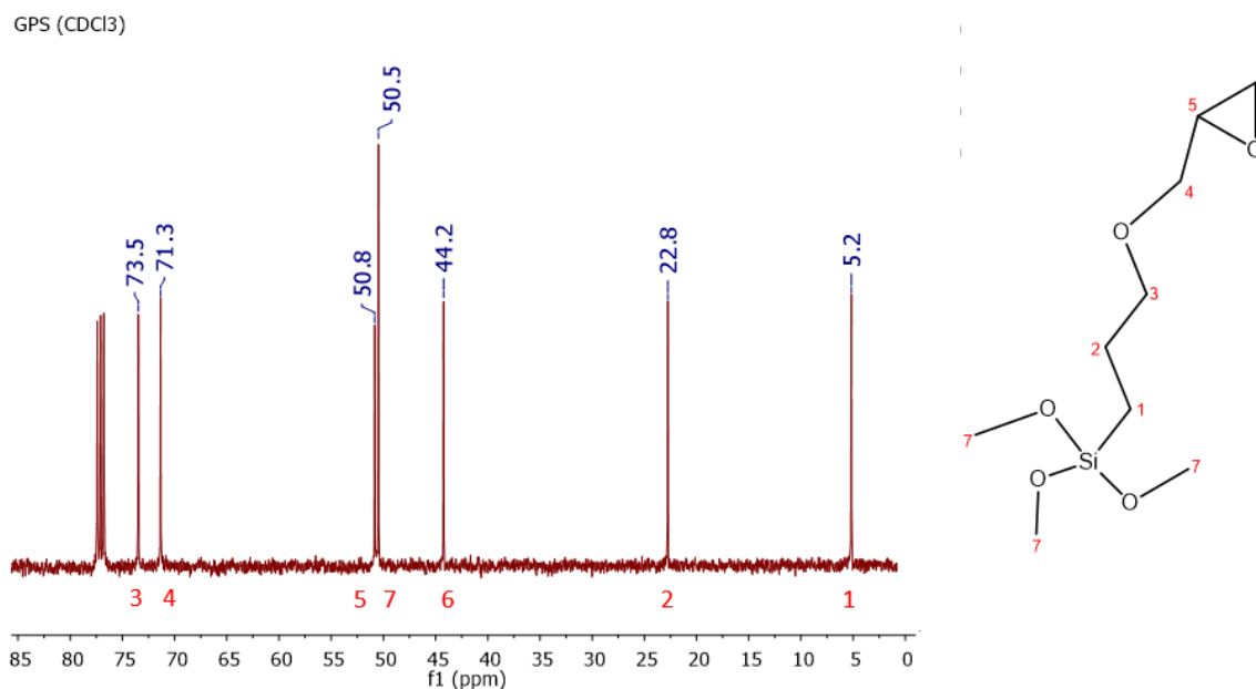
Figure II-10. 13 C NMR spectrum of GPS silane in CDCl 3 .
