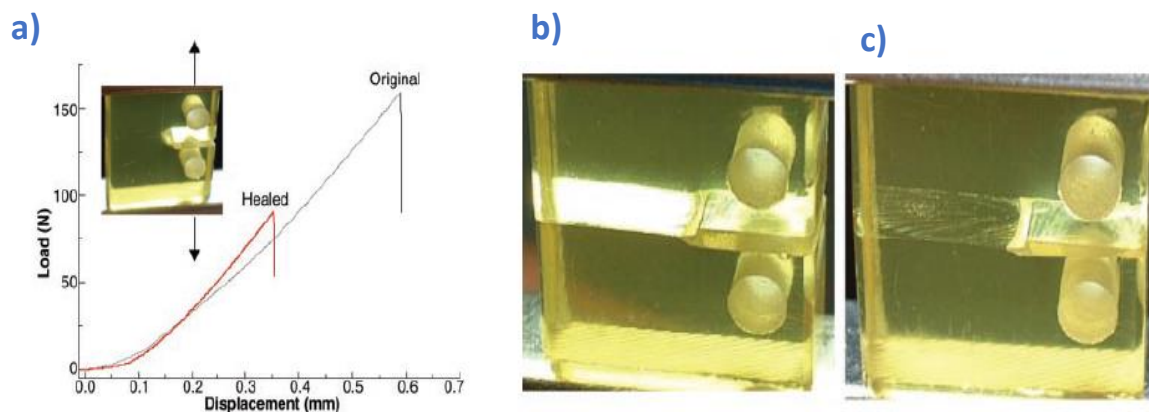
Figure I-9. Mending efficiency of polymer-based on DA and rDA reaction, a) mending efficiency obtained by fracture toughness testing of compact tension test specimens, b) broken specimen before thermal treatment, and c) specimen after thermal treatment 46 .
