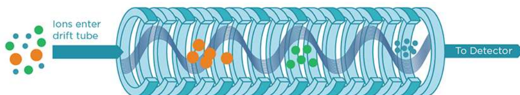
Figure II-14: Principle of traveling wave ion mobility spectrometry.
