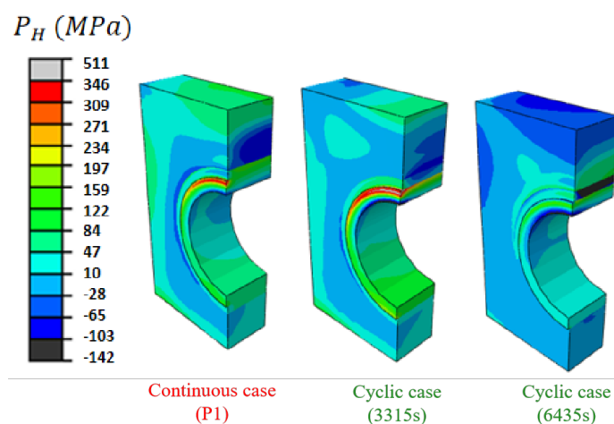
Figure 2.119: Hydrostatic stress field: 3315 s and 6435 s correspond to the end of the plateau of the 1st cycle, and the end of the cooling process, respectively (see Figure 2.117 (a)).
