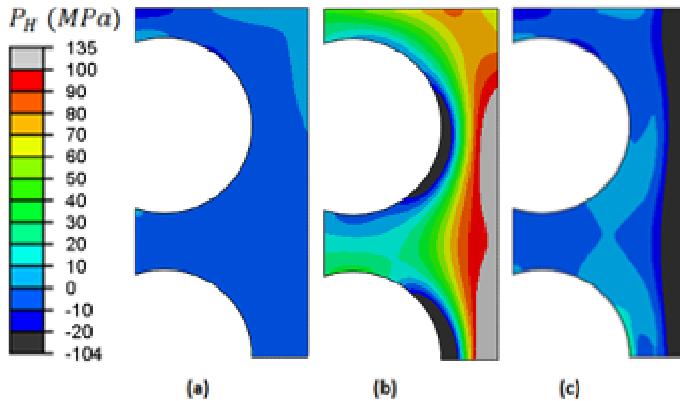
Figure 2.54: Hydrostatic pressure field at the end of Phase 1: (a) only the cooling pipes pressures are considered; with all the mechanical fields, at the higher (b) and lower exposure temperatures (c).
