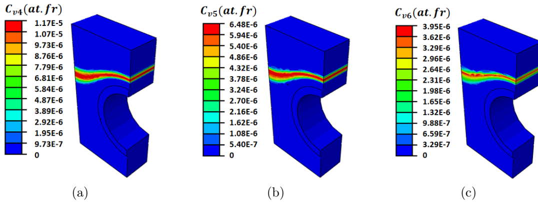
Figure 3.6: C_{V_4} \sim C_{V_6} fields at the end of the computation.
