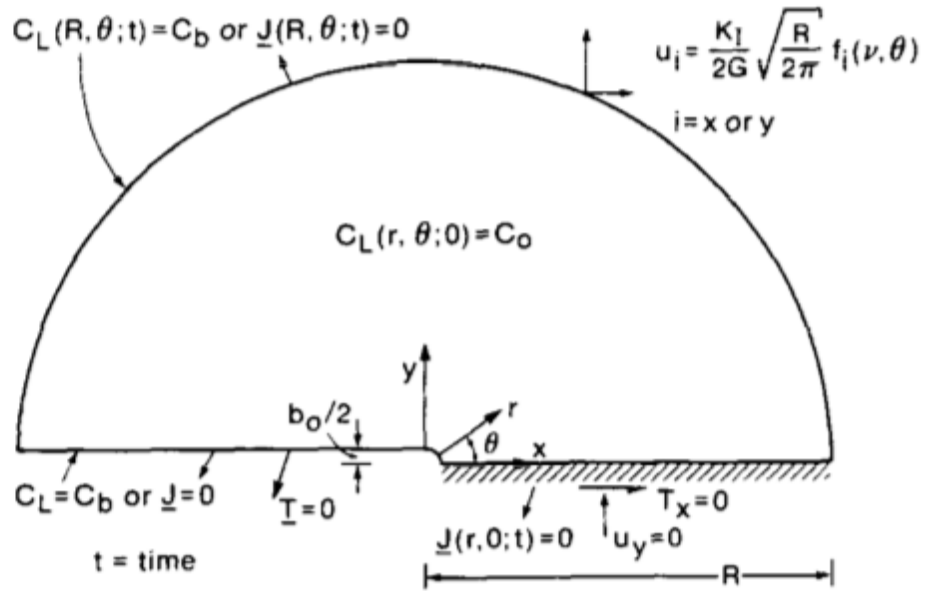
Figure 1.2: SSY configuration [17]
