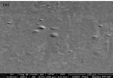
Figure 1.7: W Plansee: After pure D plasma exposure [41].
