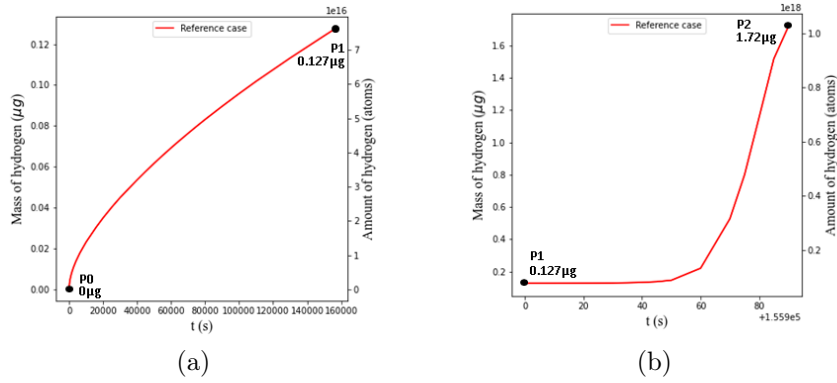
Figure 2.105: Evolution of (a) H retention evolution between P0 \sim P1, (b) H retention evolution between P1 \sim P2.
