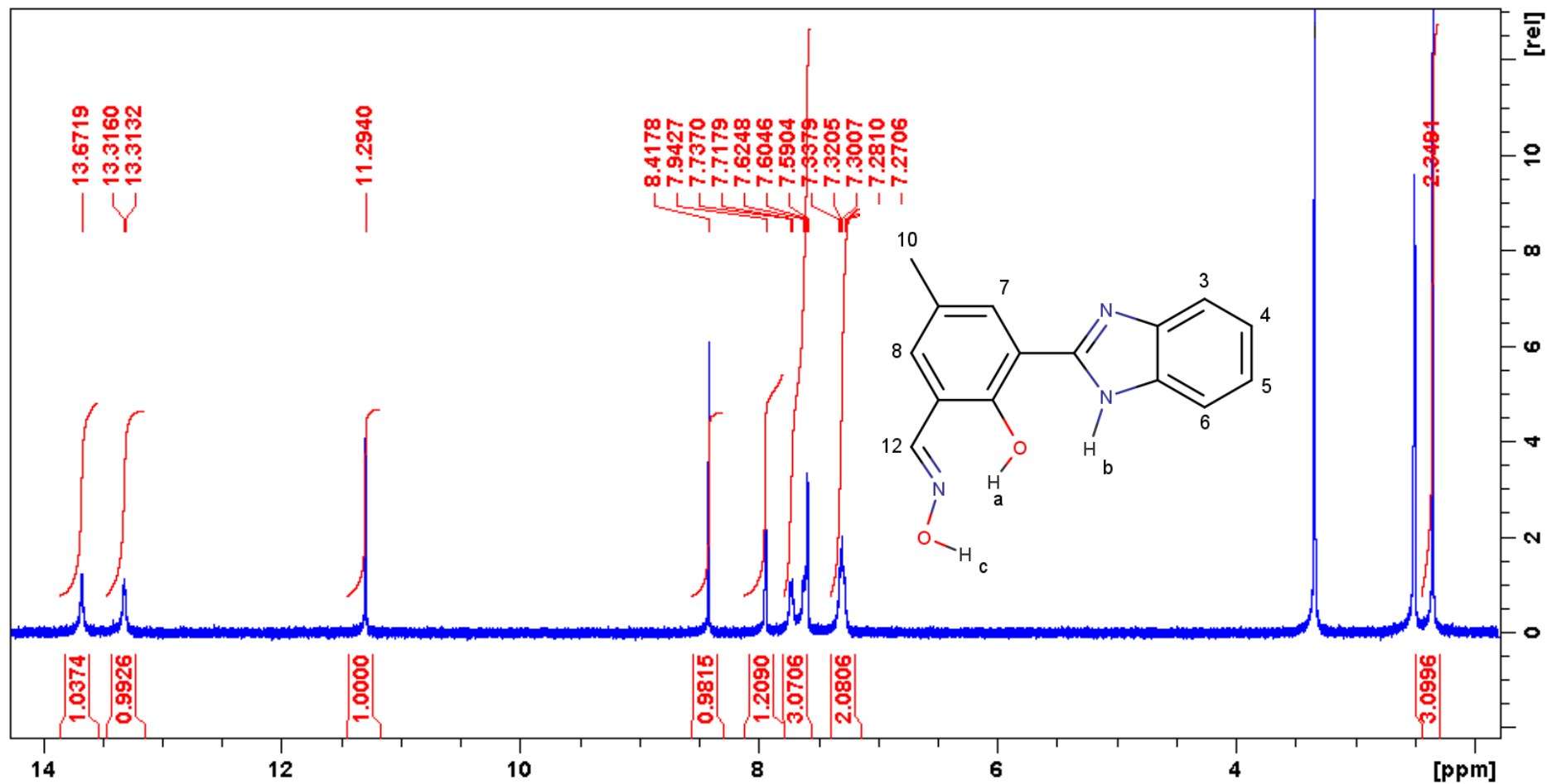
Figure 68. ^1\text{H-NMR} ( \text{DMSO-}d_6 , 400 MHz) spectrum of M4.
