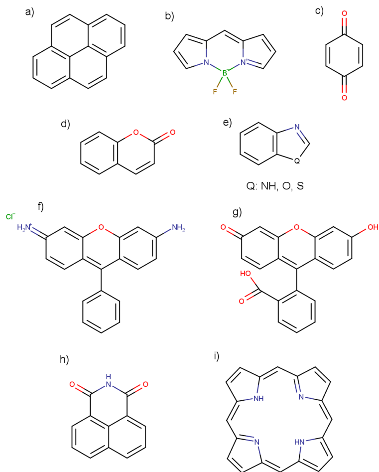
Figure 11. Chemical structures of common fluorophores: a) pyrene, b) BODIPY, c) quinone, d) coumarin, e) Q: NH, O, S, f) rhodamine, g) fluorescein, h) naphthalimide and i) porphyrin.
