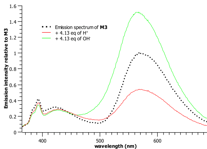
Figure 142. Emission spectra of M3 when adding acidic or basic solutions. [M3] = 12.1 \mu\text{mol/L} in THF : MeCN 0.5 : 99.5; \lambda_{\text{exc}} = 352 nm.
