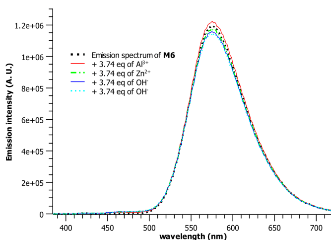
Figure 192. Comparison of the emission spectrum of M6 upon subsequent additions of 3.74 equivalents of \text{Al}^{3+} , \text{Zn}^{2+} and \text{OH}^- . [\text{M6}] = 10.7 \mu\text{mol/L} in THF : EtOH : \text{H}_2\text{O} 0.4 : 49.8 : 49.8 medium; \lambda_{\text{exc}} = 372 \text{ nm} .
