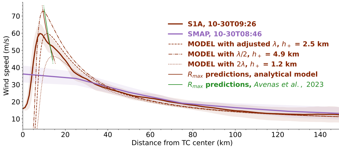
Figure 3. SAR wind profile estimate (solid thick brown curve, i.e. the second of the three SAR wind profile estimates in Fig. 1) and radiometer wind profile estimate (solid thick purple curve) collocated in time ( i.e. with a 40-min time difference) for TC Goni. For each observed wind profile, the shaded area denotes the standard deviation along each radius. Analytical model predictions (thin dashed, dotted and dash-dotted brown curves) for three different values of \lambda (see text for details) and corresponding R_{max} estimates (thin solid brown curve, obtained using an ensemble of \lambda values). For comparison, the R_{max} estimates obtained by considering steady angular momentum conservation 7 to the ensemble of analytical solutions ( i.e. the model V_{max} and outer size predictions obtained when varying \lambda ) are shown in green.
