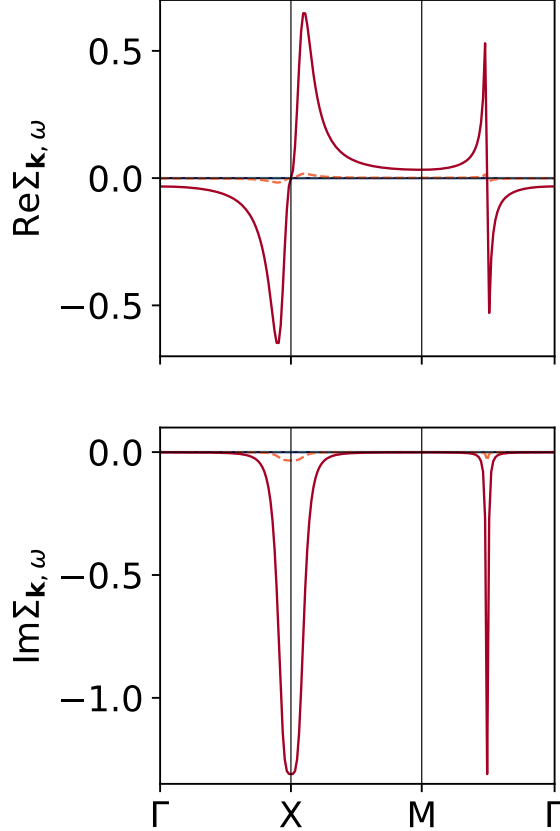
Figure 5.15: Real and imaginary self-energy \Sigma_{\mathbf{k},\omega} along the high-symmetry path \Gamma X M \Gamma at the Fermi energy calculated utilising the SCFF theory. The components are evaluated along V = U/4 in the U - V phase diagram, with a selection of values of the interaction parameters, denoted by their colours in Fig. 5.12. Note, only the self-energies associated with U \in \{1.5, 2.0\} are sufficiently large to be observed.
