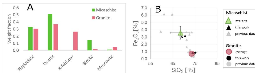
Figure III.3: Description of the two main lithologies from the Ploemur CZO: granite and micaschist. (A) mineralogical composition as reported by Béchenec et al. (2012b). (B) bulk silicon and iron contents of the two lithologies. Sub-figure (B) includes previous reported data from (Touchard; 1999) and Anne-Catherine Pierson-Wickmann (personal communication) corresponding to ICP-OES analyses on bulk powders. The dataset is completed with additional ICP-OES and X-ray fluorescence measurements made in the framework of this work.
