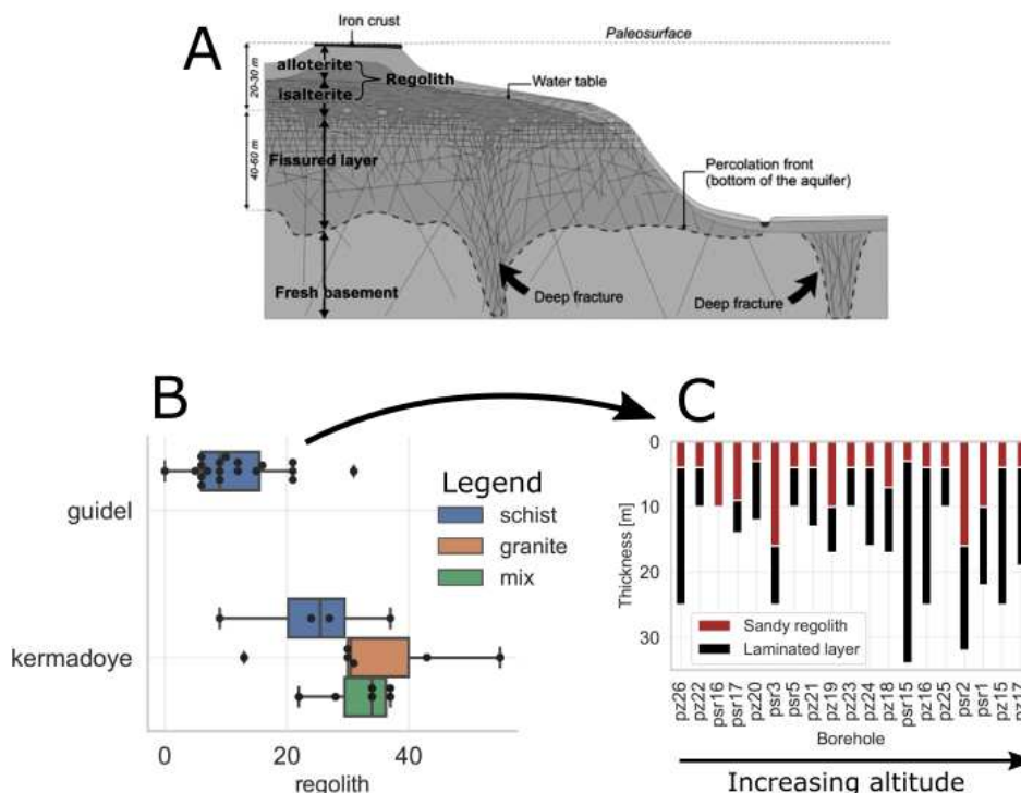
Figure III.2: Regolith structure in the Ploemur CZO. A): Idealized architecture of a fractured-bedrock aquifer from (Dewandel et al.; 2006). B): average thickness of the regolith (sandy + laminated regolith compartments) and C): detail of the regolith compartment for the Guidel catchment. Data corresponds to thickness estimations based on the borehole drilling reports.
