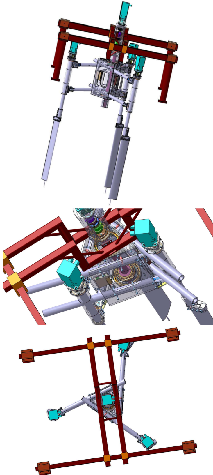
FIGURE D.2 – Architecture du prototype SHIVA
