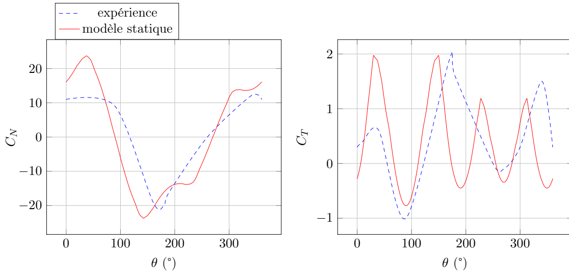
FIGURE 2.25 – Cas D : 2 pales, \lambda=5
