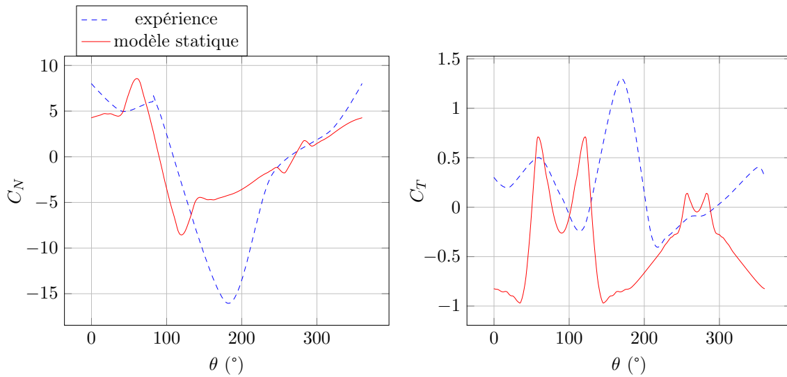
FIGURE 2.24 – Cas C : 2 pales, \lambda=2.5
