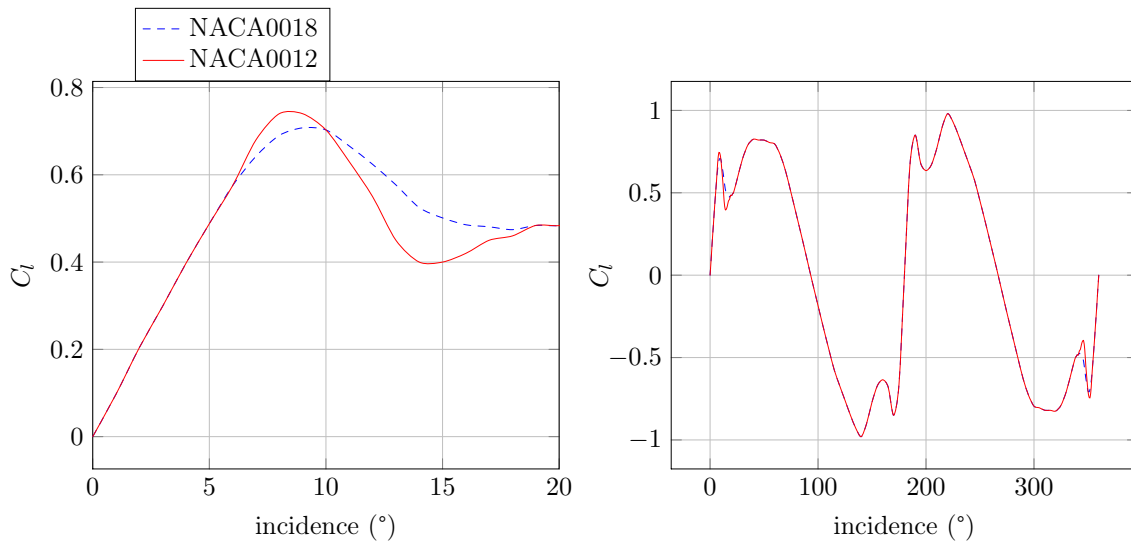
FIGURE 2.14 – Coefficients de portance [Vittecoq and Laneville 1982, Sheldahl and Klimas 1981, Paraschivoiu 1998]
