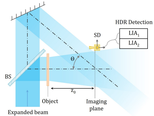
Figure V.15: Diagram of the experimental implementation for holography coherent imaging in transmission configuration, using HDR detection.
