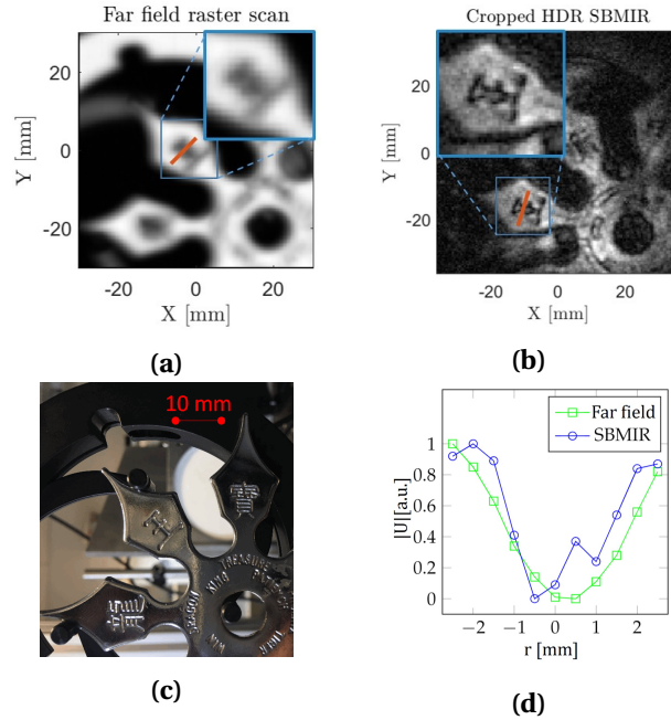
Figure V.8: (a) Amplitude distributions of the considered sample obtained through far field assessment at 287 GHz with NA = 0.25 and (b) amplitude reconstruction emerging from the SBMIR extraction on HDR measurement sets. (c) Picture of the object under inspection and (d) cross-sections of the Chinese kanji for both approaches.
