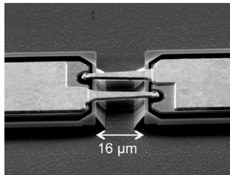
Figure I.12: SEM image of a pair of anti-parallel Schottky diodes for frequency mixing operation [73].
