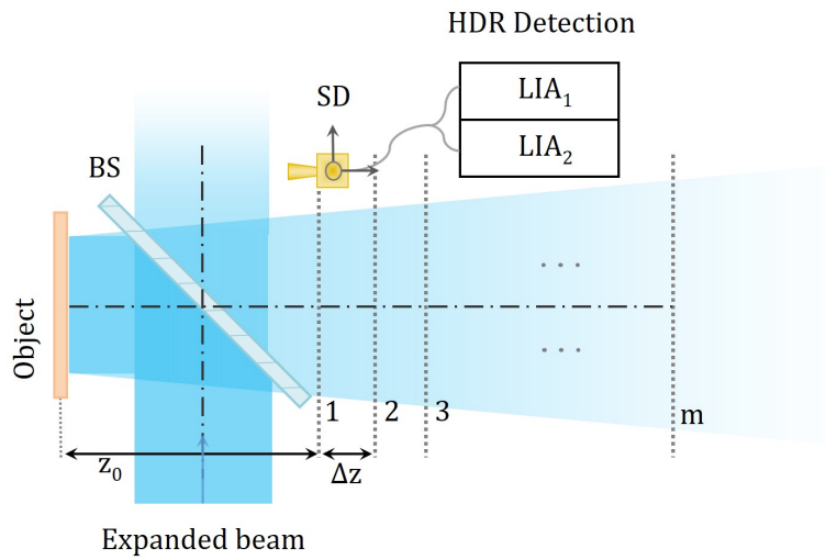
Figure V.4: Diagram of the experimental implementation for phase retrieval measurement in reflection configuration, using HDR detection.
