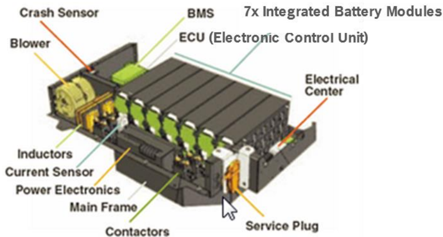
Figure 1-3 Schematic diagram of a PHEV pack manufactured by A123 Systems
