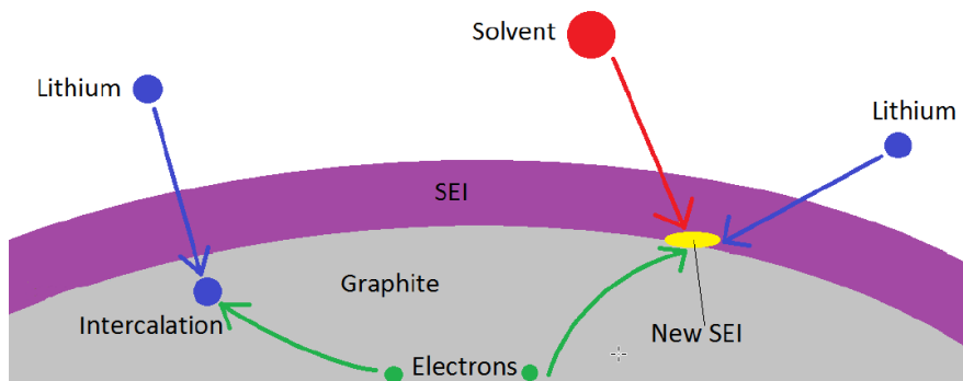
Figure 4-10 Desired intercalation reaction vs. undesired SEI formation at the interphase of anode and electrolyte [64]
