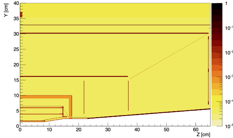
Figure 3.9: Material scan of the inner tracking region of the simulated ILD detector in units of X_0 with arbitrary absolute scaling. Figure taken from [54].
