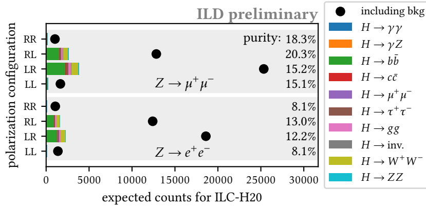
Figure 6.1: Expected number of events per Higgsstrahlung sample after the \sqrt{s} = 250\text{ GeV} runs that are planned in the ILC-H20 proposal.
