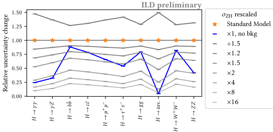
Figure 6.30: Comparison of the expected Higgs BR uncertainties for various Higgsstrahlung cross sections. Additionally, the blue graph indicates the BR uncertainties that could be achieved with perfect background separation.
