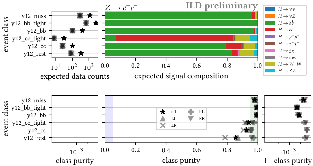
Figure 6.15: Expected event composition per class in the y12 sector. For a detailed description see Fig. 6.2.
