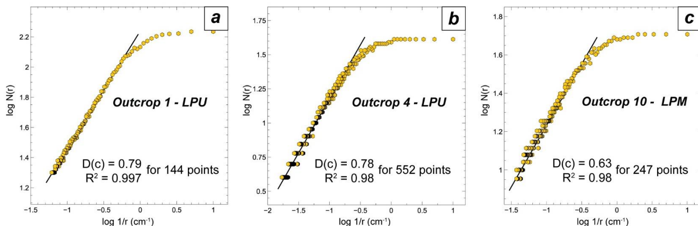
Figure IV.9: A), B), C) Vein clustering following the methodology of Manning (1994). Black lines correspond to fits with power laws for the linear part of these truncated datasets.
