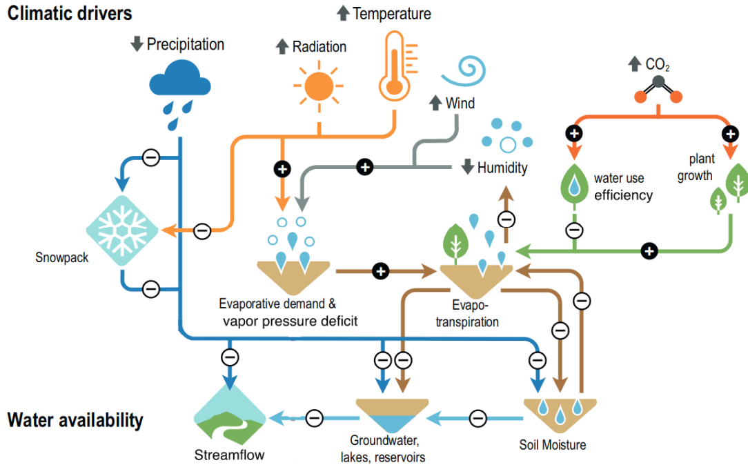
Figure 1.2 – Climatic drivers playing a role in water availability. Plus and minus signs denote the direction of change that drivers have on factors such as snowpack, evapotranspiration, soil moisture, and water storage. From Douville et al. (2021).
