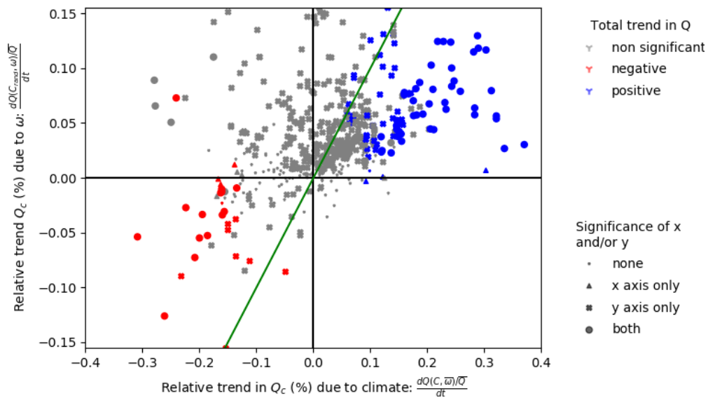
(b) "Climatic" system Q_{climat} : relative trends (% per year over the century) due to changes in \omega_c versus relative trends due to changes in climate variables C
