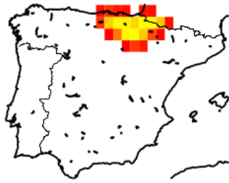
(a) Watershed of the gauging station Castejon on the Ebro river
