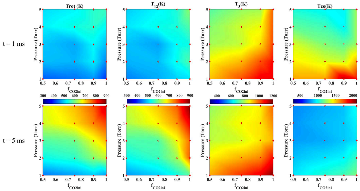
Figure 6.13: Temperature "maps" of the temperatures in the pulse at two different times: 1ms (close to the peaks) and 5ms (end of the pulse) as a function of the pressure and the initial CO 2 fraction
