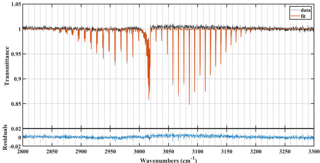
Figure 6.4: Comparison of the measured spectrum and of a simulated spectrum 4s after the beginning of the pulse during a 5ms in a 50:50 CO 2 -CH 4 discharge at 1 Torr. The simulated spectrum is at equilibrium at T=440K. The residuals are plotted below
