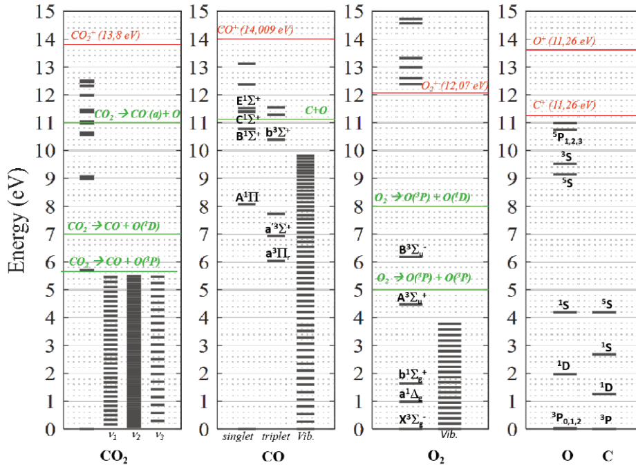
Figure 1.4: Vibrational and electronic excited levels of \text{CO}_2 , \text{CO} , \text{O}_2 and atomic \text{O} . The ionization is plotted in red and the electron impact dissociation thresholds are plotted in green
