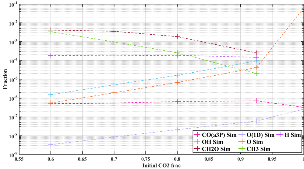
Figure 4.27: Evolution of the simulated fractions of minor species with initial \text{CO}_2:\text{CH}_4 ratio at 1.85sccm and 5Torr
