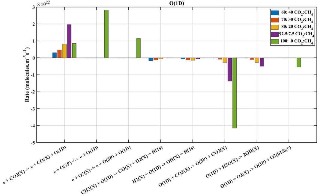
Figure 4.33: Evolution with initial mixture of the reaction rates of the main creation and destruction processes of O(1D) at pseudo-steady state at 1.85sccm, 5Torr. The positive rates represent the creation, the negative the destruction processes. Each initial mixture is plotted in a different color
