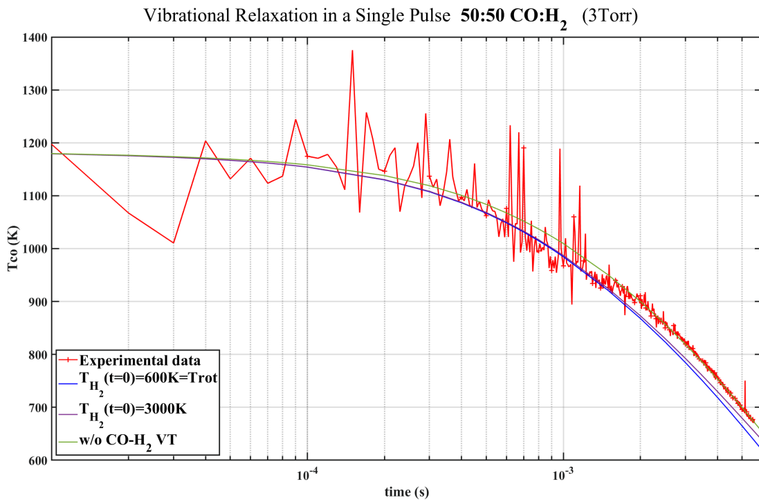
Figure 6.31: Simulation of the relaxation of T_{co} during the post-discharge of a 50:50 CO:H 2 Single Pulse experiment. the experimental T_{co} is plotted in red
