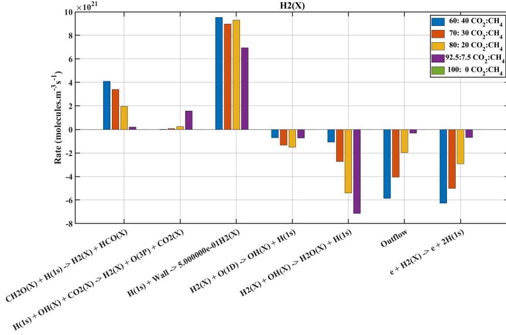
Figure 4.32: Evolution with initial mixture of the reaction rates of the main creation and destruction processes of H 2 at pseudo-steady state at 1.85sccm, 5Torr. The positive rates represent the creation, the negative the destruction processes. Each initial mixture is plotted in a different color
