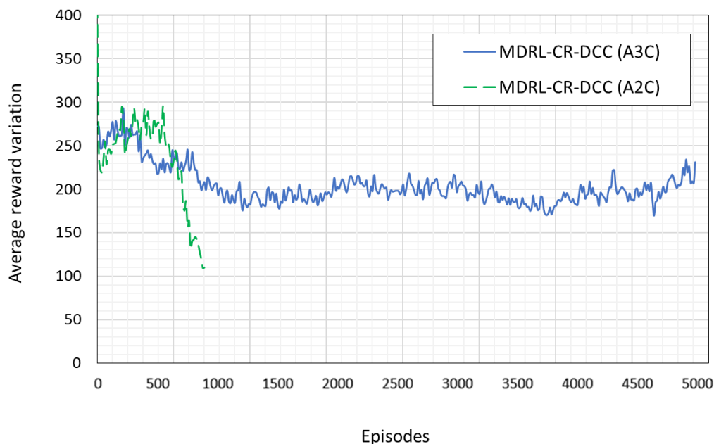
Figure 6.4 Average reward variation as a function of training episodes of the global model
