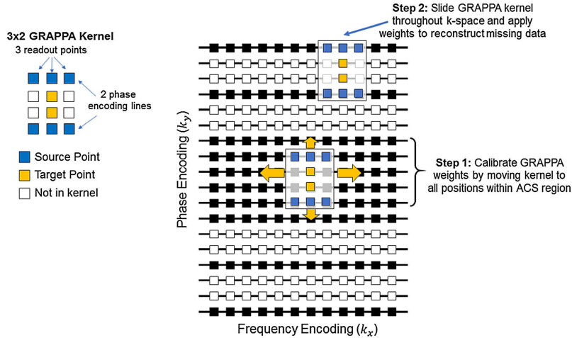
Figure 2.4: The GRAPPA reconstruction technique operates on the principle that the full k-space information from each coil can be effectively interpolated. This is achieved by utilizing an interpolation kernel, which is estimated from a fully sampled region, along with the undersampled k-space data obtained from each individual coil. (This figure is taken from [Ham17]).
