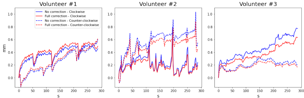
Figure B-3: Time course of motion regressors of the translation over the z-axis (estimated with SPM12) for the three volunteers and the clockwise as well as the counter-clockwise time series data.
