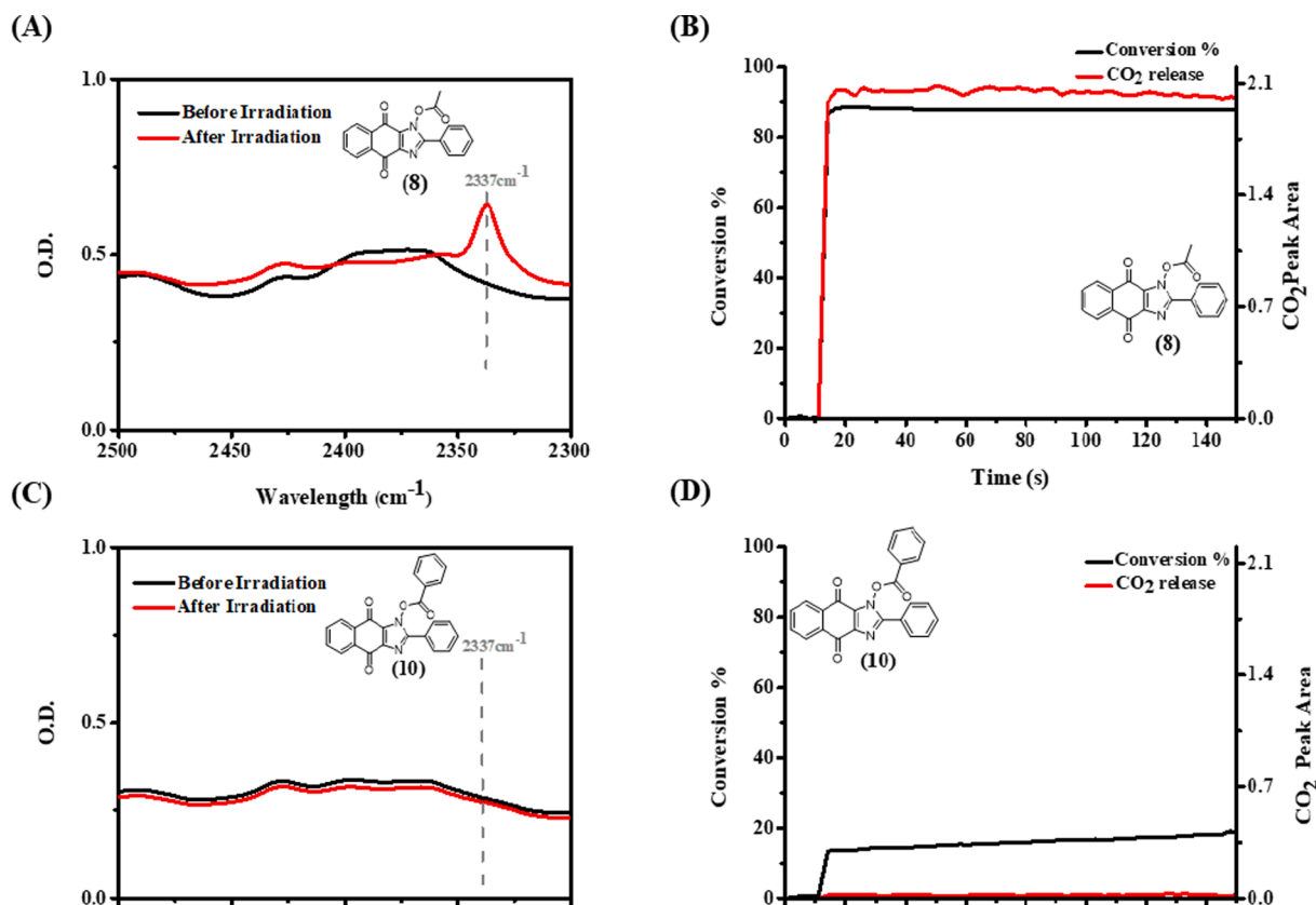
Fig. 28. (A) Detection of CO 2 released during photopolymerization using (8), (B) Decarboxylation-Conversion correlation using (8), (C) Detection of CO 2 released during photopolymerization using (10) and (D) Decarboxylation-Conversion correlation using (10); PI (0.5 % w) in TA (thin film polymerization @405 nm in laminate). Reproduced with the permission from Ref. [69].
