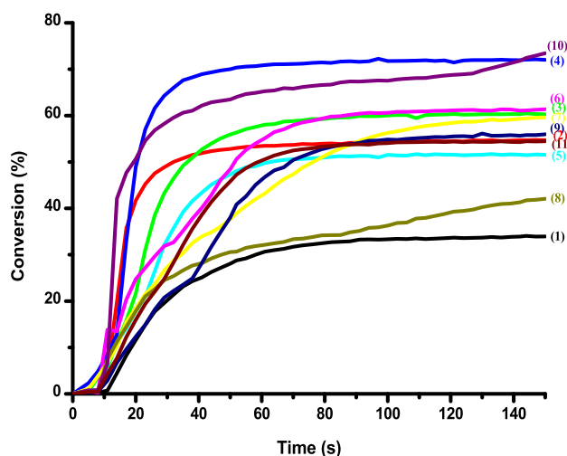
Fig. 7. Photopolymerization profiles of TMPTA (acrylate function conversion vs. irradiation time) in laminate (thickness = 25 \mu\text{m} ) upon exposure to LED light \lambda = 405 nm in the presence of: (1) OXE-A (0.5 % w); (2) OXE-B (0.5 % w); (3) OXE-C (0.5 % w); (4) OXE-D (0.5 % w); (5) OXE-E (0.5 % w); (6) OXE-F (0.5 % w); (7) OXE-G (0.5 % w); (8) OXE-H (0.5 % w); (9) OXE-I (0.5 % w); (10) OXE-J (0.5 % w); and (11) OXE-K (0.5 % w); respectively. The irradiation starts after t = 10 s. Reproduced with the permission from Ref [42].
