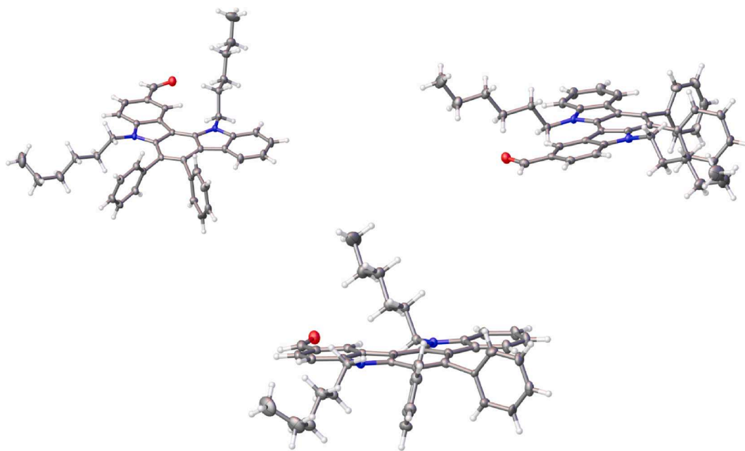
Fig. 2. Crystal structure of C3.
