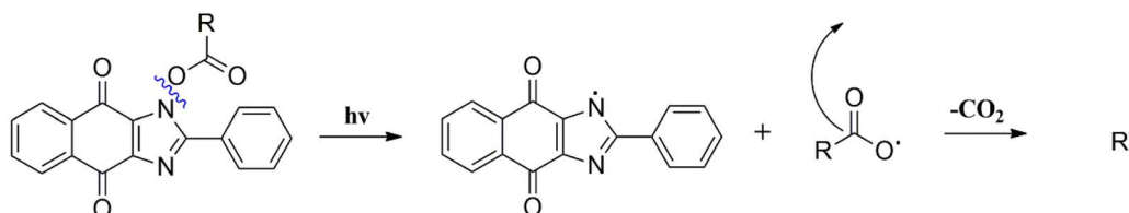
Scheme 4 Proposed photochemical mechanisms for naphthoquinone-based imidazolyl esters.
