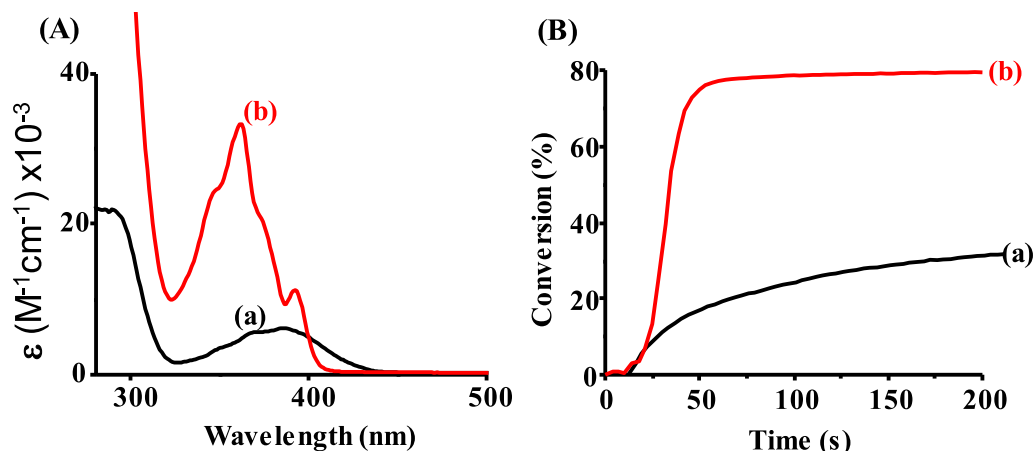
Fig. 24. (A) UV-visible absorption spectra of (a) An-OXE 2 and (b) Py-OXE 2. (B) Photopolymerization profiles of acrylates functions using (a) An-OXE 2 (0.5 % w) and (b) Py-OXE 2 (0.5 % w) as photoinitiators. Reproduced with permission of Ref. [59].
