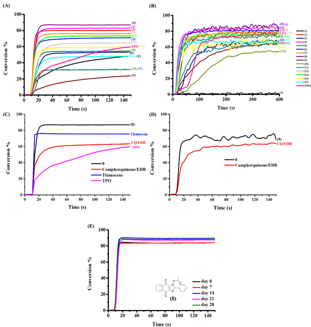
Fig. 4 Photopolymerization profiles of TA (acrylate function conversion vs. irradiation time) using different photoinitiators (0.5 wt%) in (A) laminate (thickness = 25 μm) and (B) under air (thickness = 1.4 mm) upon exposure to a LED light ( \lambda = 455 nm). (C) Photopolymerization profiles of TA in laminate (thickness = 25 μm) with: compound (8) (0.5% w/w), CQ/EDB (0.5%/0.5% w/w); TPO (0.5% w/w) and titanocene (0.5% w/w). (D) Photopolymerization profiles of UDMA in laminate (thickness = 25 μm) with: compound (8) (0.5% w/w), CQ/EDB (0.5%/0.5% w/w) and (E) photopolymerization profiles of TA using compound (8) (0.5% w/w) for different storage times in TA monomer. The irradiation starts at t = 10 s.
