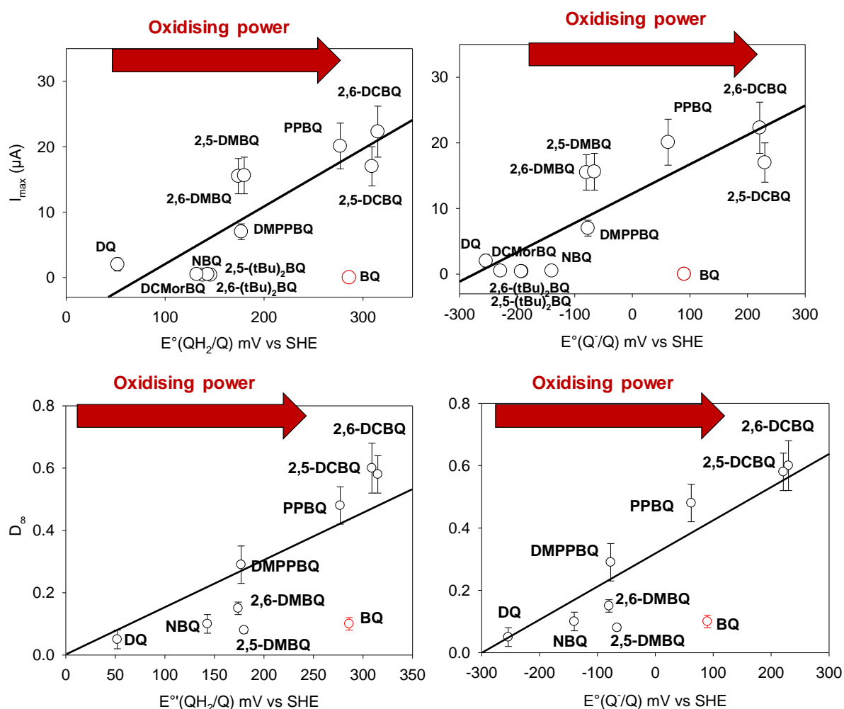
Figure 1. Summary of the main results mentioned in article n°1 : I_{\max} = f(E^\circ) ; D_\infty = f(E^\circ) for different quinones.
