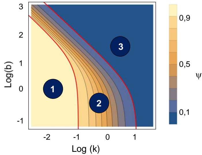
Figure 23. 3D-Zone diagram calculated from electrochemical experiments for the tandem \Delta\text{petA} algae/2,6-DCBQ. \psi is the normalized steady state photocurrent. k is an undimensionnal parameter that compares the rates of Q reduction and \text{QH}_2 oxidation. b is related to the electron harvesting step and especially on the ratio of the mass to charge transfer rates.
