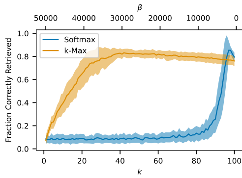
(a) MNIST with Euclidean similarity
