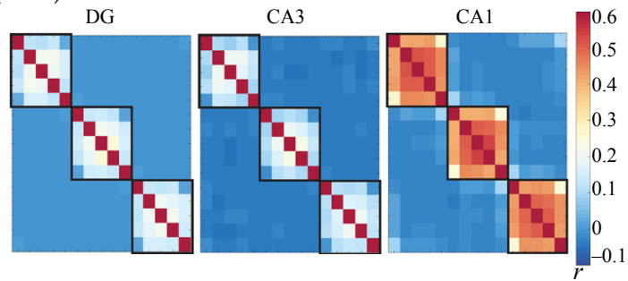
(d) Settled response of the model proposed by Ketz et al. (2013) in a simulation of the community structure task performed by Schapiro, Turk-Browne, M. M. Botvinick, et al. (2017). The symmetric heatmaps show the average representational similarity for each node pair of the graph depicted in Figure 4.7a. The diagonal represents the correlation between nodes with themselves. Adapted from Schapiro, Turk-Browne, M. M. Botvinick, et al. (2017).
