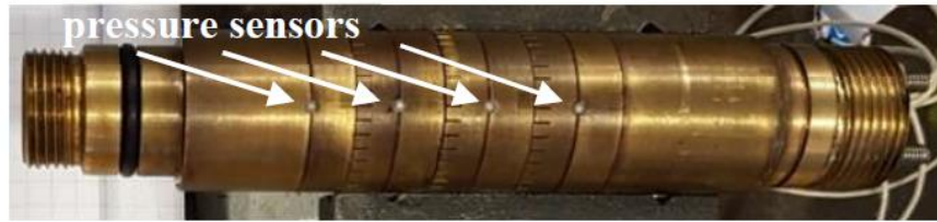
Figure 39: Multisensor device
