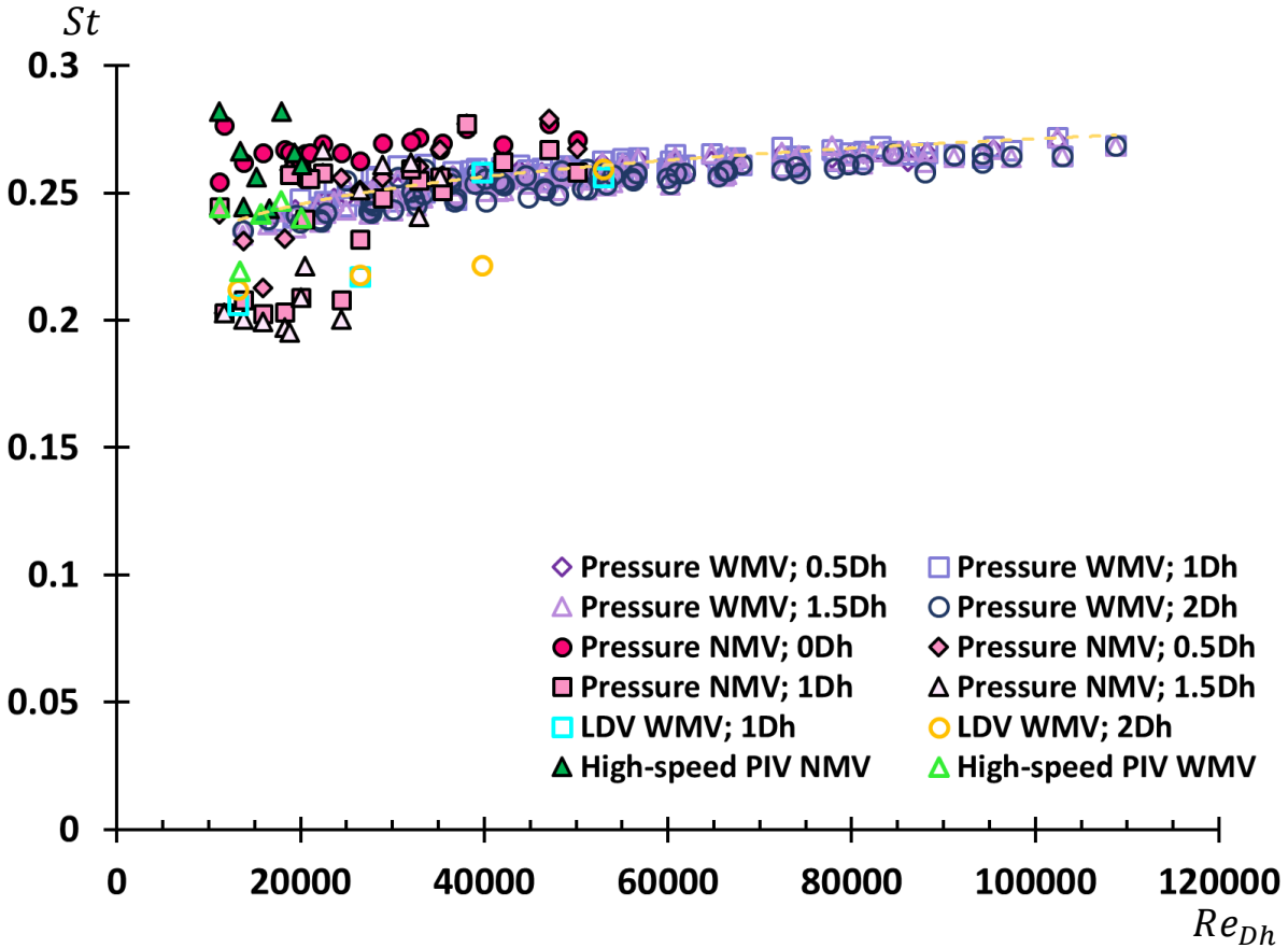
Figure 103. Strouhal-Reynolds Map
