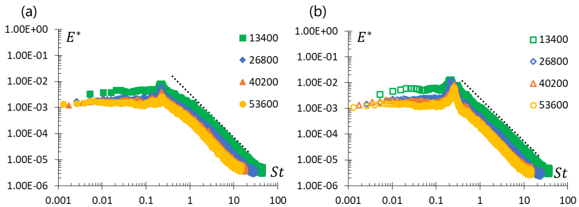
Figure 94: LDV velocity spectra of (a) spring and (b) dimple at y/D_h = 1 for Re_{D_h} = 13400, 26800, 40200, 53600
