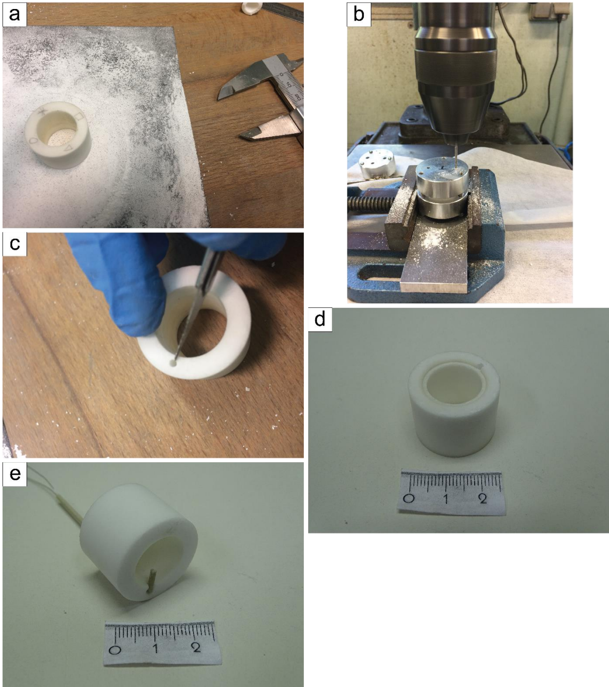
Figure VII.9. (a) The outer salt pieces are grinded with sandpaper to obtain the right length. (b) The bottom outer salt piece is drilled in order to pass the thermocouples inside. (c) The top part of the drill is dug with a scalpel to receive the 90° angle of the thermocouples. (d) At the bottom part of the bottom salt piece there is a special trench that will fit the small Cu disc. (e) The thermocouples should fit well inside the trench dug at the top part of the outer bottom salt piece.
