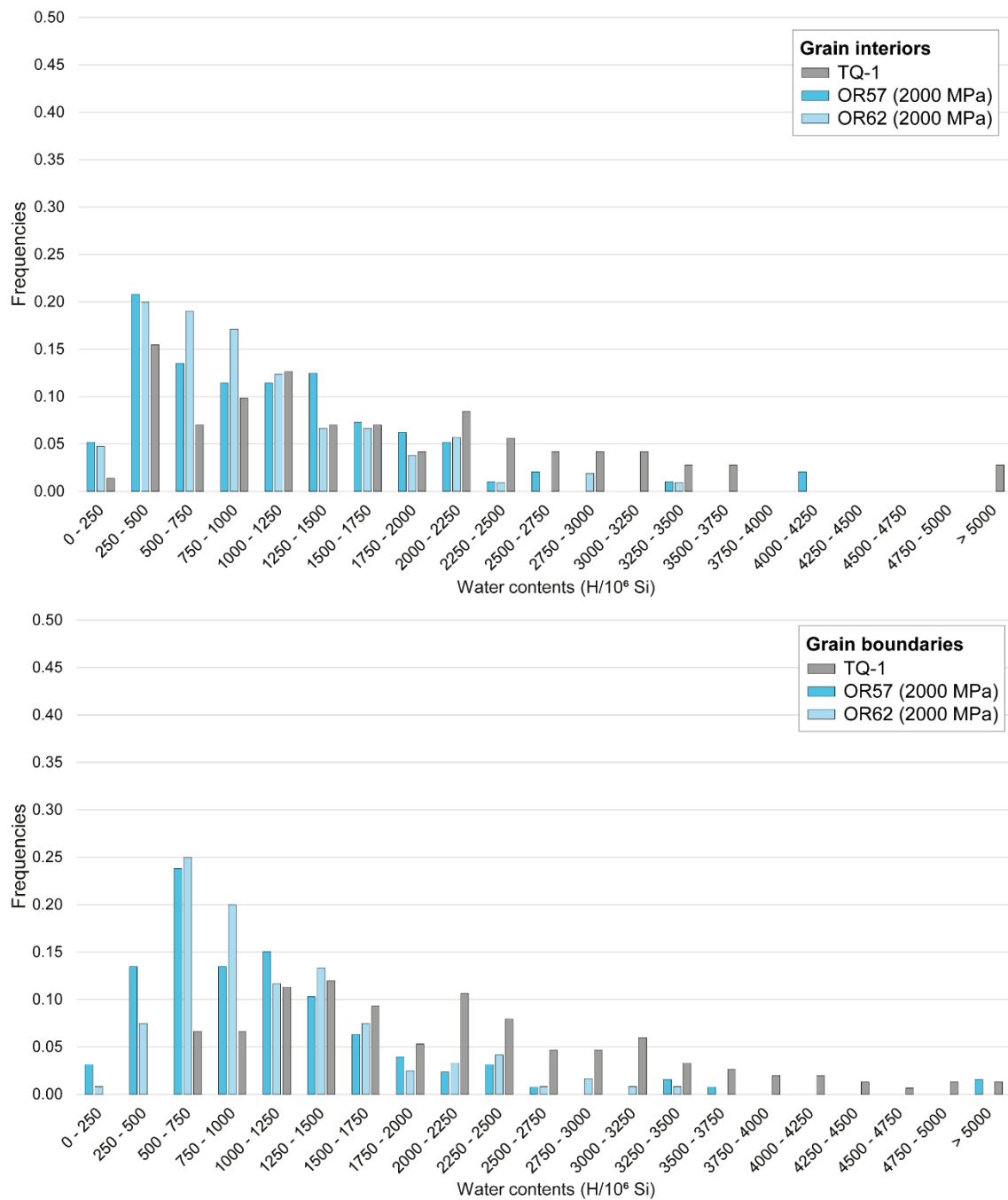
Figure IV.13. H 2 O contents distributions for grain interiors and grain boundaries (H/10 6 Si) for samples OR57 and OR62 deformed at 2000 MPa confining pressure and starting material sample TQ-1. The deformed samples show lower dispersion and higher grouping in the low H 2 O content values.
