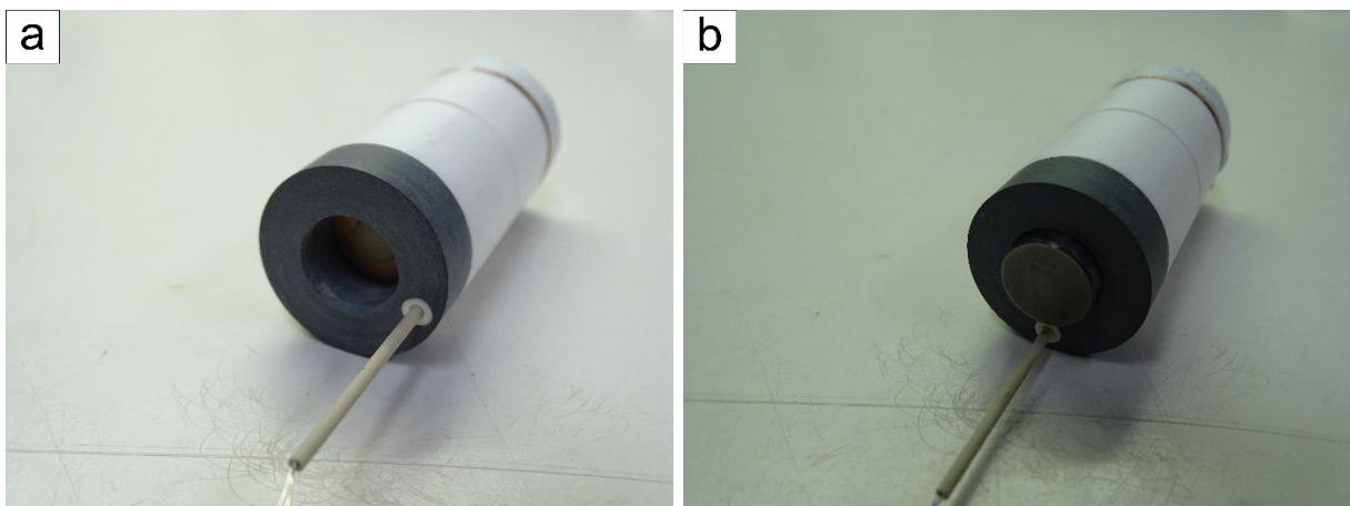
Figure VII.16. (a) The pyrophyllite bottom piece is put at the very bottom of the assembly. The thermocouple (mullite tube) being inserted into the crushable alumina. (b) The tungsten carbide plug is placed into the pyrophyllite piece.
