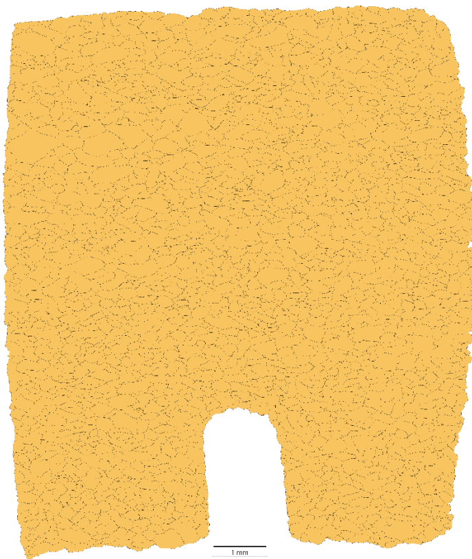
Figure VII.23. Segmentation of optical light microscopy mosaic image of deformed sample OR52 (700 MPa) and corresponding statistics for quartzite grain sizes, aspect ratio and major axis orientation.
