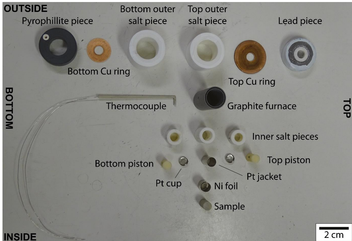
Figure II.2. Sample assembly "écorché" showing all the pieces that constitute it. These pieces go on the Tullis-modified Griggs apparatus.
