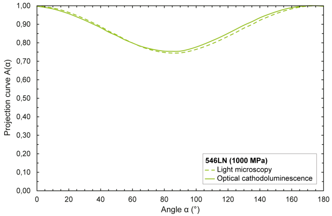
Figure VII.32. SURFOR projection curves for deformed sample 546LN (1000 MPa). The sample presents a strain of 24.6% at 85° for sand grains (LM-CL) and 25.5% at 85° for quartzite grains (LM-LP).
