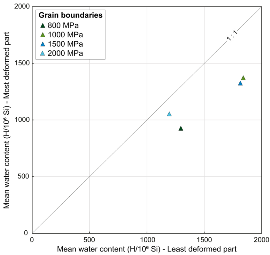
Figure IV.15. Mean H 2 O contents (H/10 6 Si) of the least deformed parts against most deformed parts in samples showing a strain partitioning.
