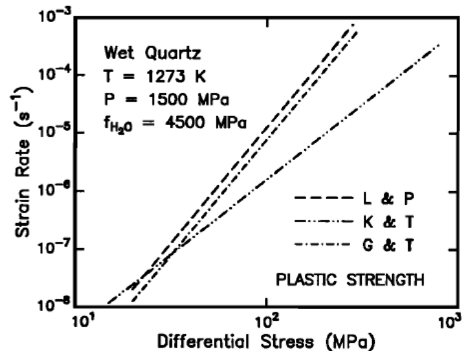
Figure 1.7. Plot of strain rate as a function of differential stress for wet quartzite. The differential stress increases with the strain rate, Kohlstedt et al. (1995).
