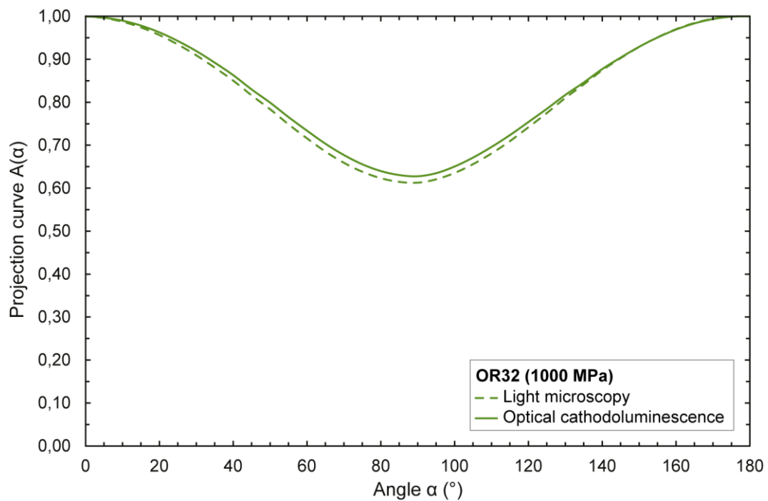
Figure VII.35. SURFOR projection curves for deformed sample OR32 (1000 MPa). The sample presents a strain of 37.2% at 90° for sand grains (LM-CL) and 38.7% at 90° for quartzite grains (LM-LP).
