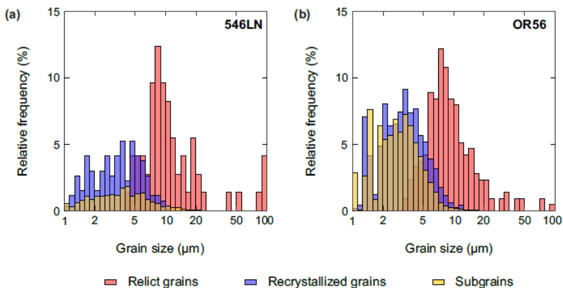
Figure III.24. \log_{10} grain size distributions for samples (a) 546LN and (b) OR56. Grain size distributions are separated into relict, recrystallized and subgrain populations.
