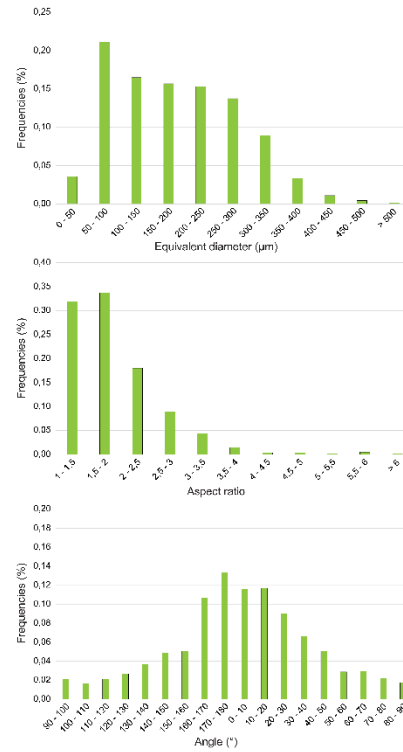
Figure VII.30. Segmentation of optical light microscopy mosaic image of deformed sample 546LN (1000 MPa) and corresponding statistics for quartzite grain sizes, aspect ratio and major axis orientation.
