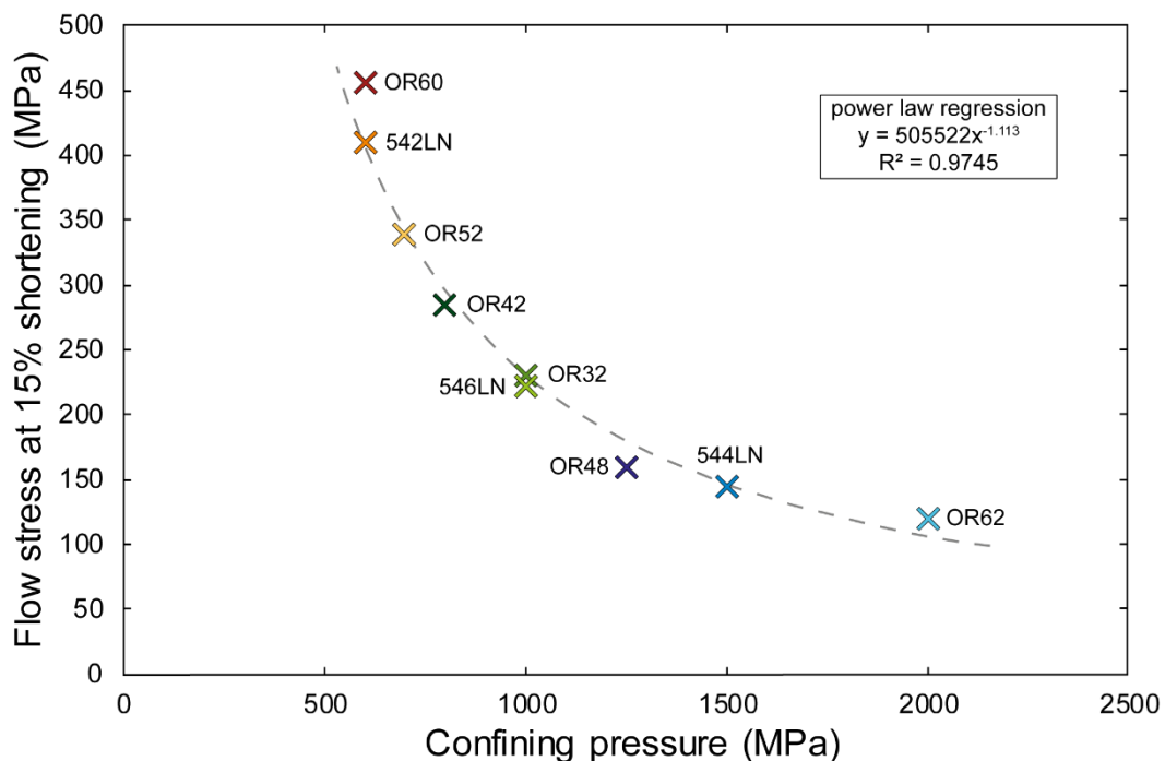
Figure III.25. A power law relationship connects the flow stresses (taken at 15% strain) and the confining pressures.
