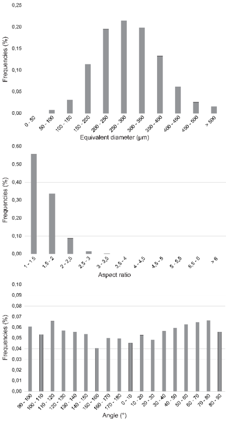
Figure VII.19. Segmentation of optical light microscopy mosaic image of starting material TQ-1 and corresponding statistics for quartzite grain sizes, aspect ratio and major axis orientation.
