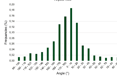
Figure VII.28. Segmentation of optical cathodoluminescence mosaic image of deformed sample OR42 (800 MPa) and corresponding statistics for sand grain sizes, aspect ratio and major axis orientation.
