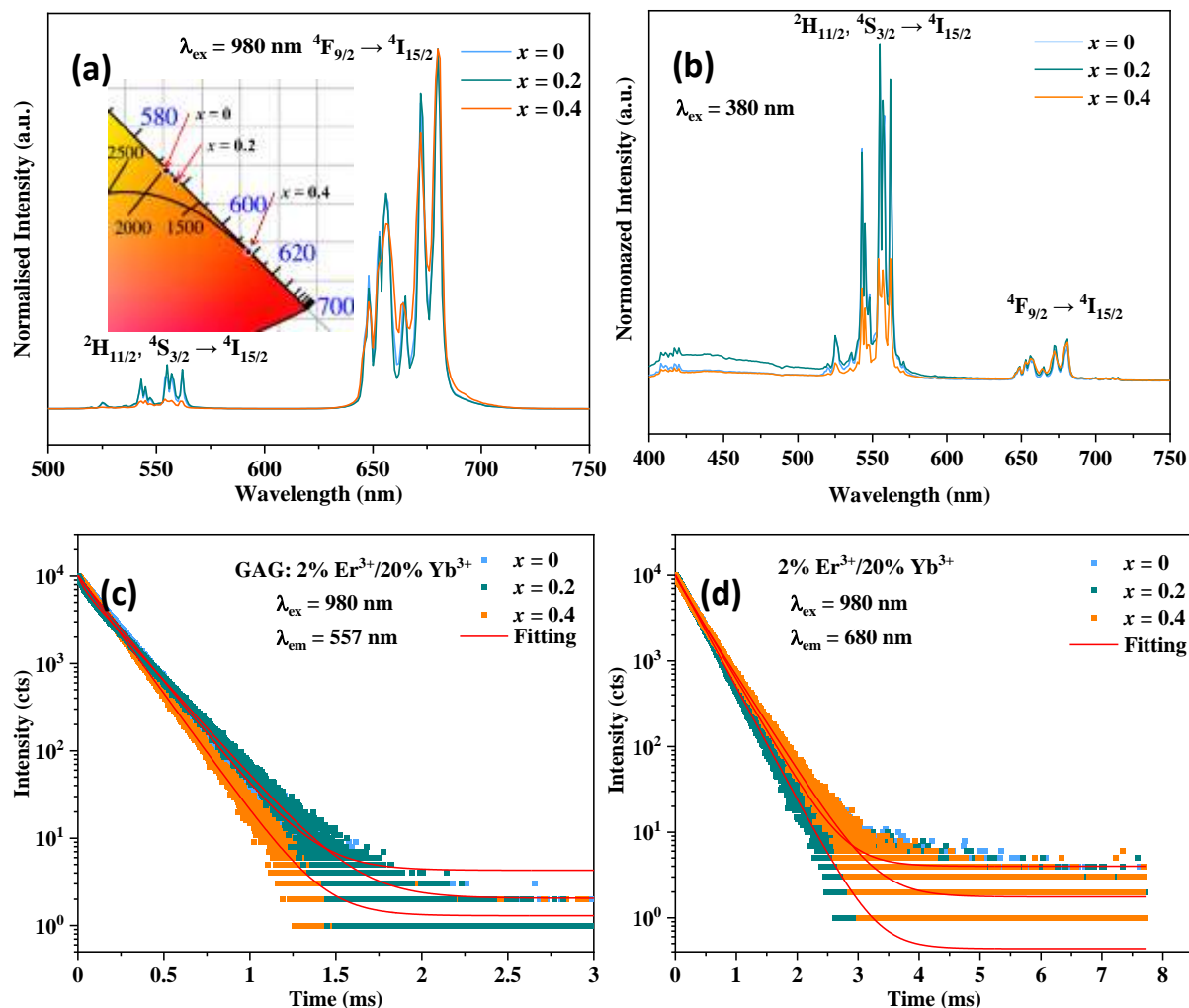
Fig 2.20 Luminescence performance of Gd_{3+x}Al_{5-x}O_{12} ( x = 0, 0.2, 0.4 ): co-doped 2% Er^{3+} /20% Yb^{3+} polished bead measured at room temperature. (a) Up-conversion emission spectra (CIE chromaticity inset) under excitation at 980 nm. (b) Emission spectra of Er^{3+} under excitation at 380 nm. (The intensity of all spectra are normalised by the highest peaks) Decay curves of Er^{3+} (c) 557 nm and (d) 680nm emission peak.
