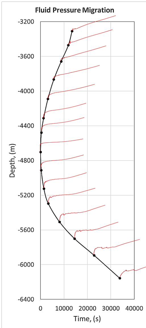
Figure 4.42. Pressure front migration from injection point at about 4.7 km to the top and bottom of the fracture for the fracture with shear slip; the left-hand side figure is plot of WHP build-up onset time versus depth of measuring points on which the red curves are WHP variation in time determined using the process explained in figure 4.14. The right-hand side sub-figures are illustration of upward and downward velocity functions along the fracture where the both profiles obey a power-law function, but the exponent of downward function is 0.4 compared to 0.5 of upward one
