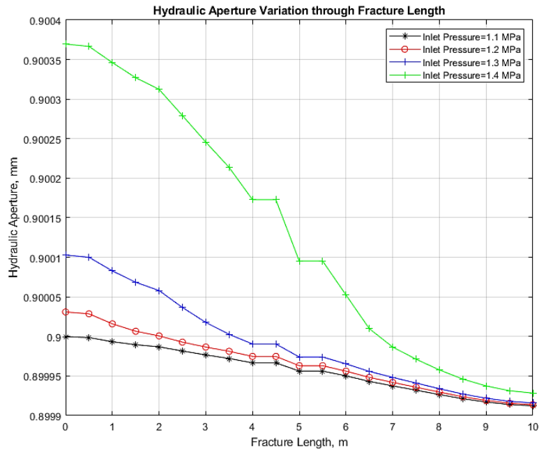
Figure 3.16. Numerical hydraulic aperture of the fracture for various magnitudes of inlet fluid pressure
