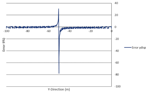
Figure A1.14. Numerical (upper) and analytical (middle) lateral displacement magnitudes in Y-direction and corresponding error (lower) in Polyaxial Stresses case
