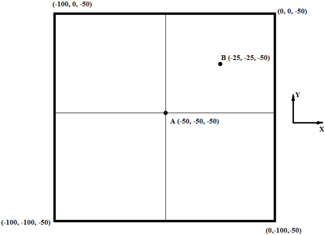
Figure 2.8. Plane view of the block of benchmarking modeling at the depth of -50 m where A and B are the points in which, respectively, the vertical and both lateral components of displacement are evaluated and compared with analytical values
