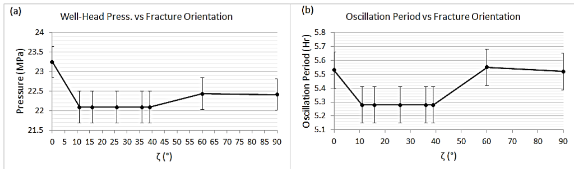
Figure A2.10. WHP (a) and oscillation period (b) variations versus different angles between fracture strike and direction of the maximum horizontal stress
