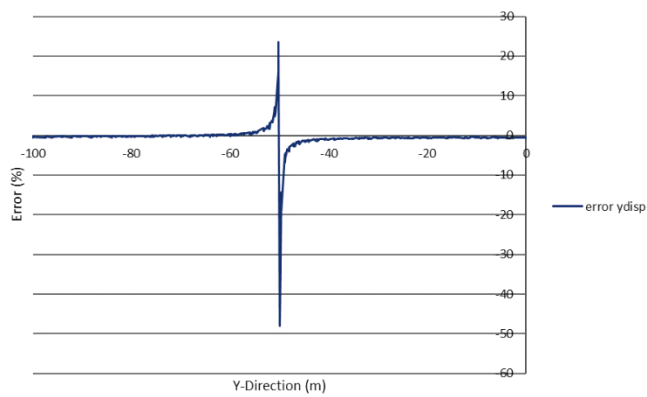
Figure A1.10. Numerical (upper) and analytical (middle) lateral displacement magnitudes in Y direction and corresponding error (lower) in Uniaxial Stress case
