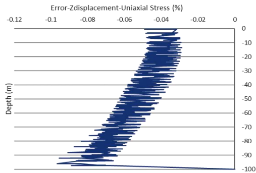
Figure A1.1. Numerical (upper) and analytical (middle) vertical displacement magnitudes and corresponding error (lower) in Uniaxial Stress case
