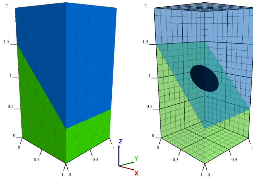
Figure 5.37. Parallelepiped block (1x1x2 m 3 ) with embedded circular finite fracture (black circular surface with diameter of 0.5 m)
