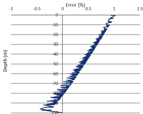
Figure 2.7. Numerical (upper) and analytical (middle) vertical displacement magnitudes and corresponding error (lower) for Uniaxial Stress case when gravity is considered
