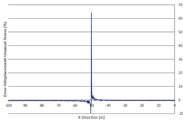
Figure A1.2. Numerical (upper) and analytical (middle) lateral displacement magnitudes in X-direction and corresponding error (lower) in Uniaxial Stress case
