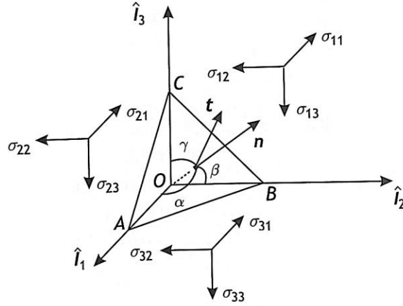
Figure 4.4. Cauchy tetrahedron used to determine stress vector components on a surface element with orientation of \mathbf{n} based on stress tensor components (Cornet, 2015)
