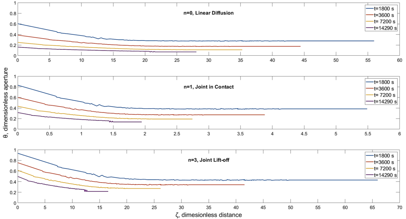
Figure 4.28. Dimensionless aperture profile versus dimensionless distance from injection point for numerical results derived from 3DEC for constant flow rate case; the graphs are drawn for all three cases of n = 0, 1 , and 3 at different times to clearly observe the opening migration along the fracture. Comparison of these plots with figure 4.27 reveals the similarity of propagation distance between 3DEC results (1.5 to 2 in all time spans) at middle graphs ( n=1 , Joint in Contact) with that of n = 1 case of Murphy et al., 2004, shown in figure 4.27 where the dimensionless distance is just over 1.5
