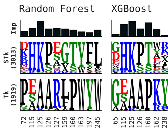
Figure 4.2: A sequence logo of the TkST sequences at top-10 selected positions selected by RF and XGB.
