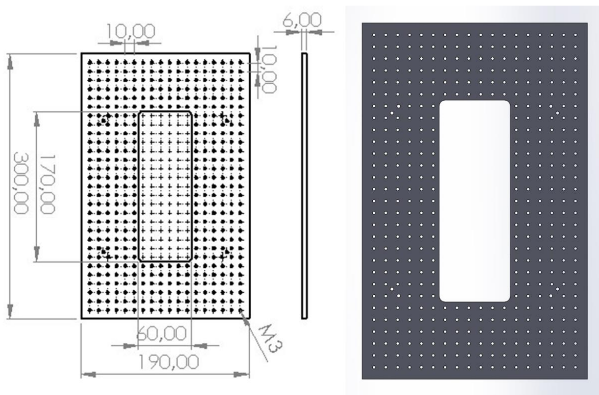
Figure 3.28 Design of the top plate after modifications (quotations are in mm).
