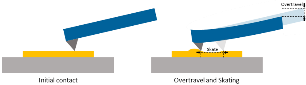
Figure 1.5 Representation of the overtravel and the skating of a probe tip.
