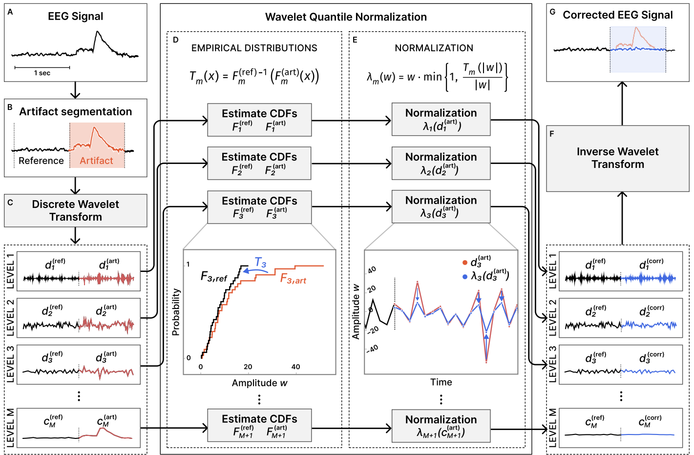
Figure 6.2 Diagram of proposed artefact removal method. A Input EEG signal (single-channel). B Artefact segmentation. C Decomposition with DWT on M levels. D Estimation of empirical cumulative density functions and transformation T_m (equation 6.9). E Normalization of wavelet coefficients (equation 6.10). F Reconstruction from corrected wavelet coefficients (equations 6.11 to 6.13). G Artefact-corrected EEG signal.
