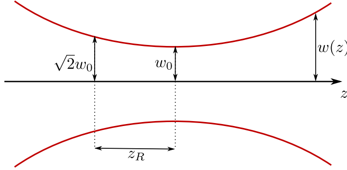
FIGURE 1.1: Gaussian beam.
