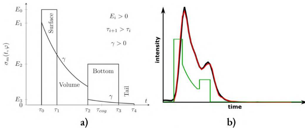
Figure 2.7: Illustration of the waveform decomposition method proposed in Schwarz et al., 2019: a) model with 10 parameters E_0 \dots E_3, \tau_0 \dots \tau_4 and \gamma to estimate; surface and bottom are modelled by boxcars to account for beam spreading caused by off-nadir incidence; effects from the water volume are modelled by two exponential segments; the tail below the bottom takes care of late echoes, likely caused by multiple scattering; \tau_{cog} is the centre of gravity of the bottom and tail segments with respect to \tau_2 (Schwarz et al., 2019). b) Illustration of the application of this method in Richter et al., 2021.
