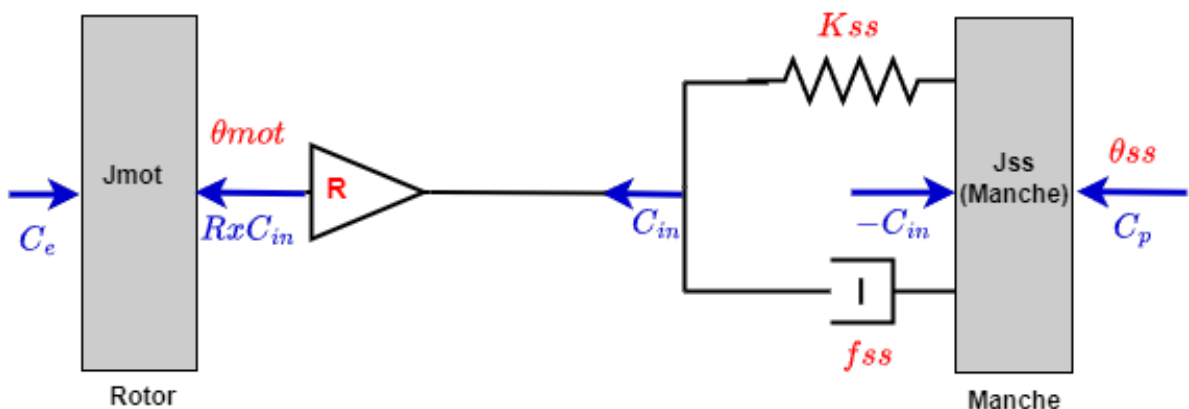
FIGURE 4.14 – Système masse-ressort
