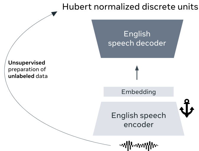
Figure 4.5. – Speech decoder training. We train an embedding-to-unit decoder in an unsupervised way. Raw speech is encoded in the sentence embedding space with a frozen speech encoder and the unit decoder is trained to recover the HuBERT units of the input speech.
