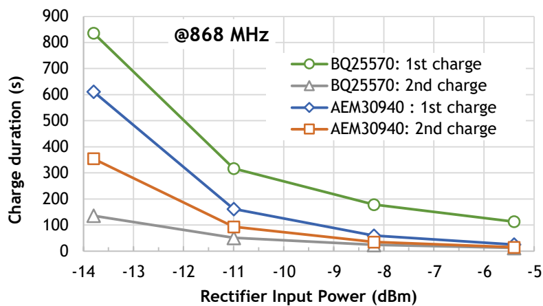
Figure III.19. Charge duration of the BSN1 using an 868 MHz rectifier for different selected PMU.
