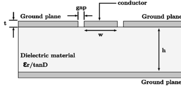
Figure IV.19. Cross section view of Coplanar waveguide with ground transmission line geometry.
