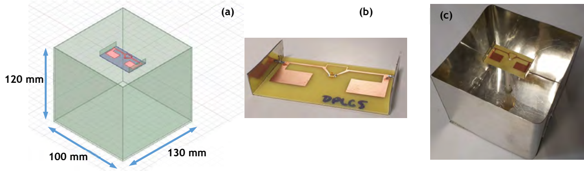
Figure III.6. Simulation design and photo of the manufactured prototype of the antenna with and without the metal cavity.
