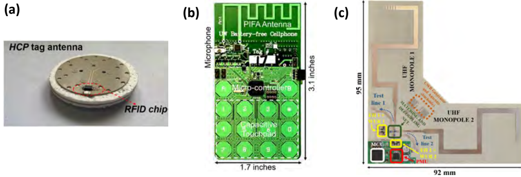
Figure I.2. Examples of developed wireless battery-free devices in the state of the art : (a) Miniaturized and Highly Sensitive Epidermal RFID Sensor for Reliable Skin Temperature Monitoring [32]; (b) First battery-free cellphone from Washington University [36]; (c) Dual-monopole UHF/UWB battery-less tag [39].
