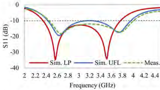
Fig. 10. Comparison of the simulated and measured return loss of the printing antenna.
