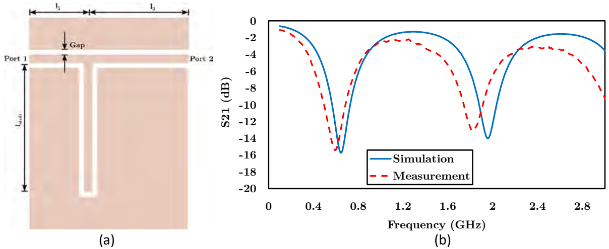
Figure IV.20. (a) Structure of the designed CPWG quarter-wavelength open-ended stub resonator; (b) Comparison between the measured and retrosimulated transmission coefficient of the CPWG open-ended T-stub resonator with \epsilon_r = 3.5 .
