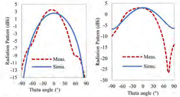
Fig. 12. Comparison of the measured and simulated radiation pattern in the E-plane ( \Phi = -90^\circ ) at 2.45 GHz (left) and 3.41 GHz (right).
