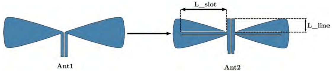
Figure V.9. Geometry of the proposed UWB Bowtie antenna. The final value of the parameters after optimization and co-simulation is L_{\text{slot}} = 16 \text{ mm} and L_{\text{line}} = 4.6 \text{ mm} .
