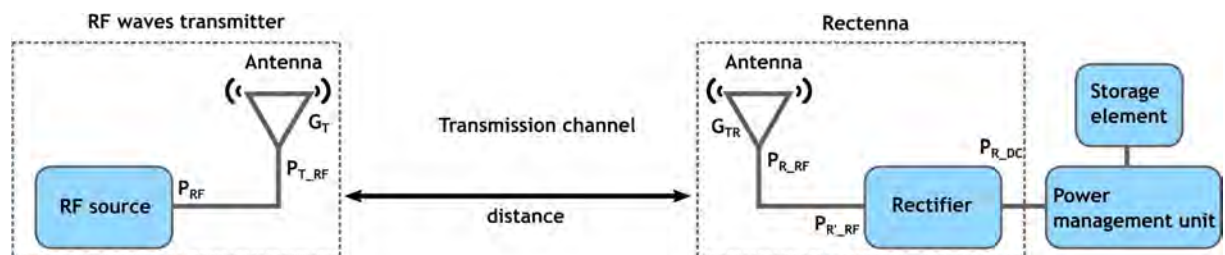
Figure I.6. Architecture of a conventional far-field WPT system.
