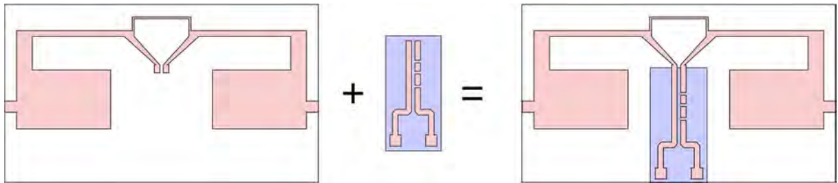
Figure II.19. Formation of the R1_3D rectenna with the antenna connected to the rectifier. Top layer of the rectenna on pink and bottom layer representing the ground plane on purple.
