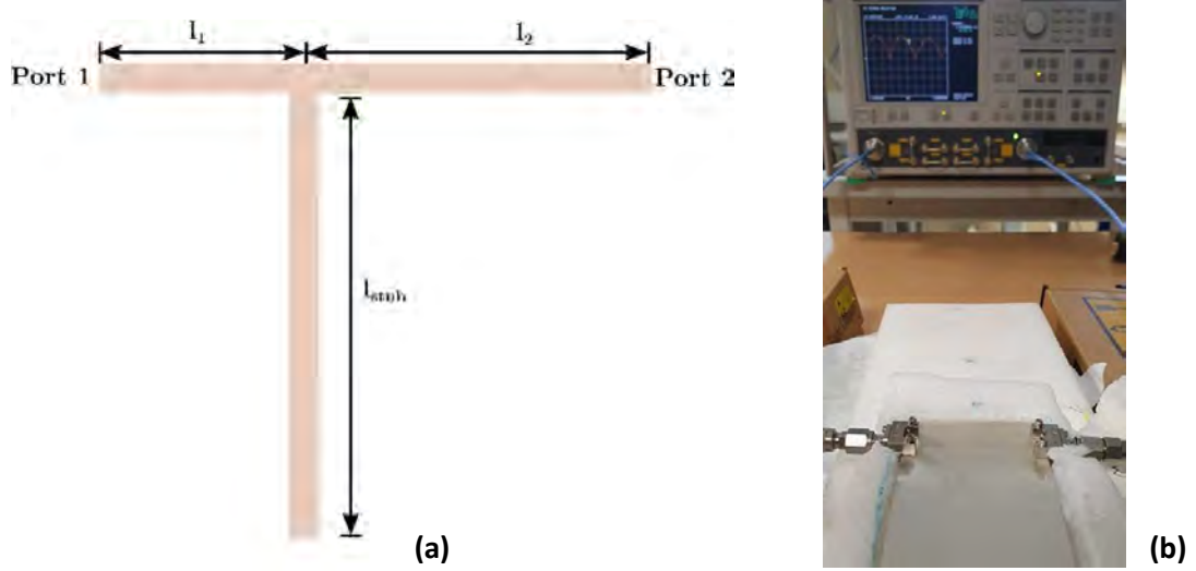
Figure IV.17. (a) Structure of the designed microstrip quarter-wavelength open-ended stud resonator ( l_1 = 15 mm and l_2 = 35 mm); (b) Photo of the S-parameters measurement setup for the prototyped structure.
