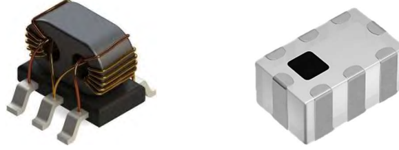
Figure IV.7. Examples of SMD Transformer Balun. (a) Balun coil with ferrite core assembled with SMD pads; (b) SMD balun transformer.
