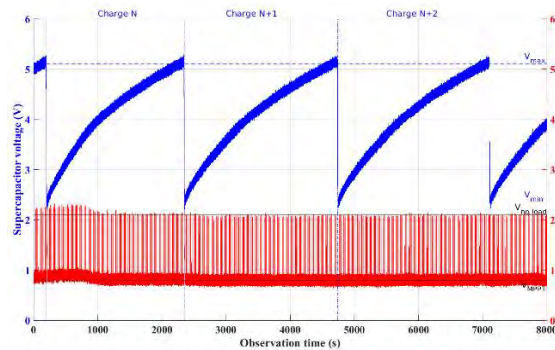
Figure III.11. Voltage waveforms at the ports of the super capacitor (blue upper curve) and rectenna output voltage (red lower curve) for a +32 dBm EIRP power.
