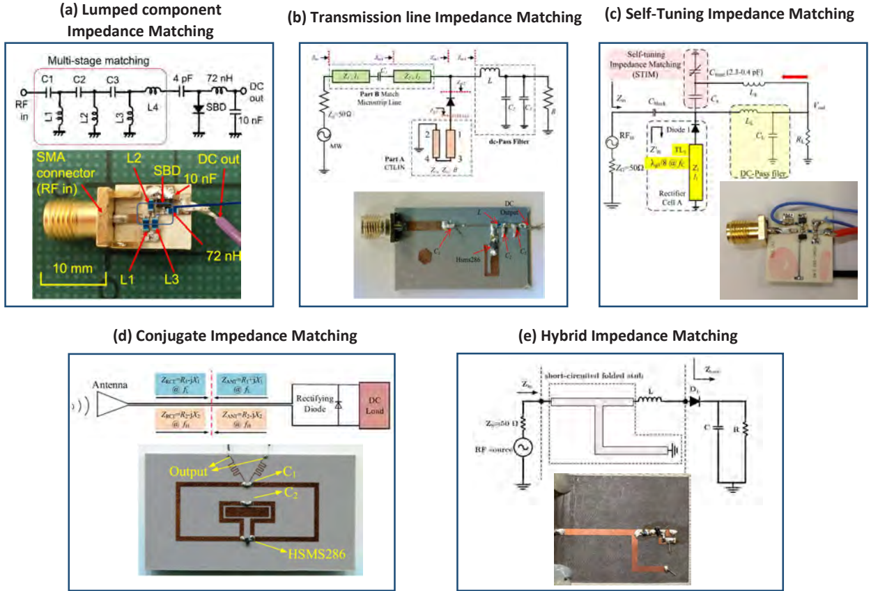
Figure I.8. Rectifier design based on different impedance matching techniques: (a) Lumped component impedance matching [84]; (b) Transmission line impedance matching [89]; (c) Self-tuning impedance matching [97]; (d) Rectenna based on conjugate impedance matching [98]; (e) Hybrid impedance matching network based on SMD inductor and short circuited folded stub [65].
