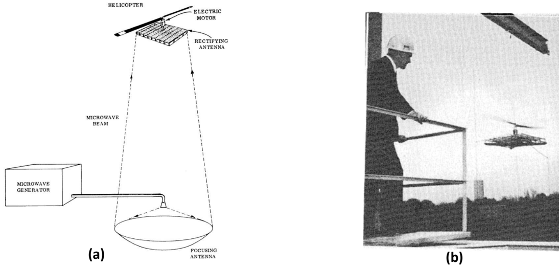
Figure I.5. (a) The basic elements of a microwave-powered helicopter system, (b) Microwave-powered helicopter in flight 60 ft above a transmitting antenna.
